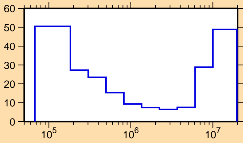
\Delta\sigma/\sigma vs. E for ^{104}\text{Tc}(n,\text{inel.})
