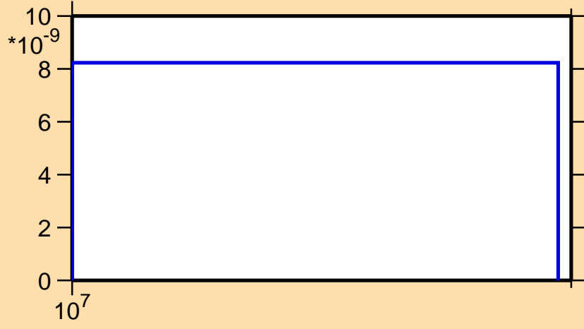
\sigma vs. E for ^{104}\text{Tc}(n,nt)
