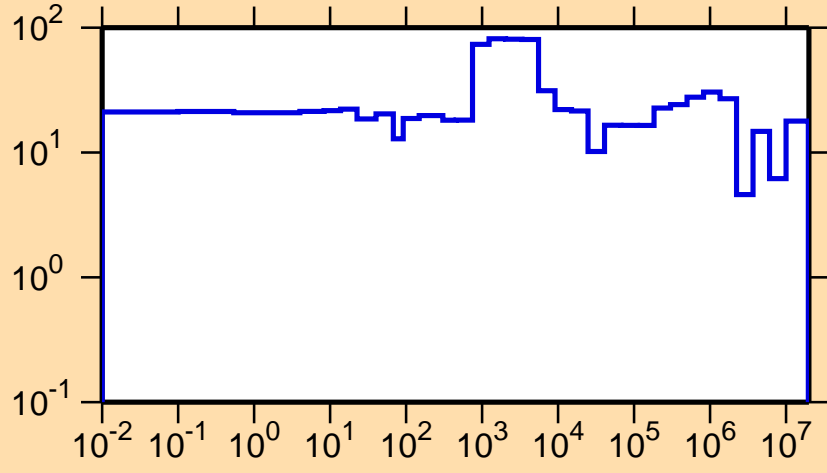
\Delta\sigma/\sigma vs. E for ^{104}\text{Tc}(n,\text{el.})
