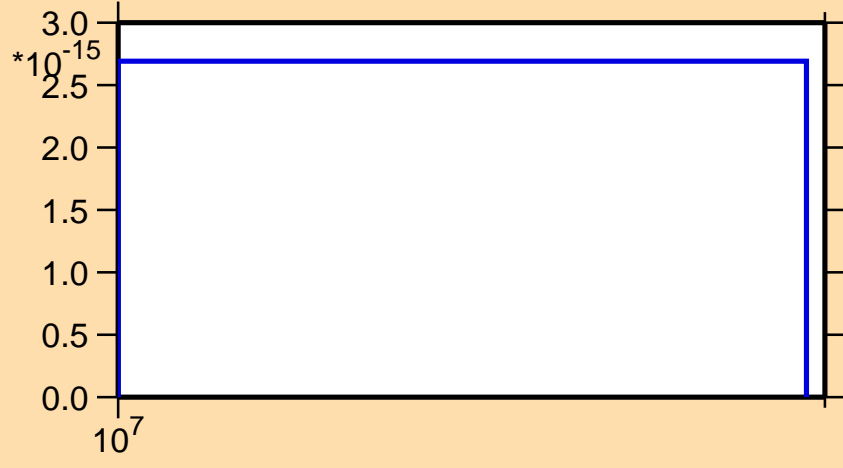
\sigma vs. E for ^{104}\text{Tc}(n,\text{He3})
