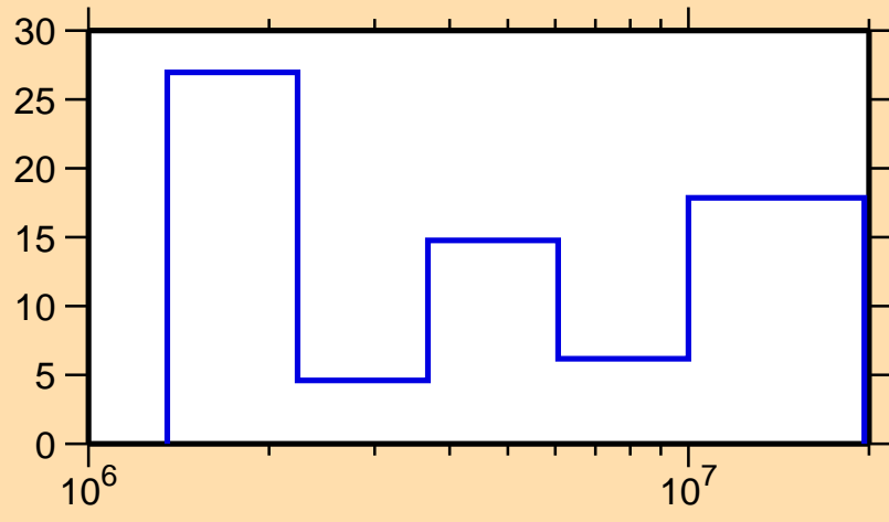
\Delta\sigma/\sigma vs. E for ^{104}\text{Tc}(n,\text{el.})
