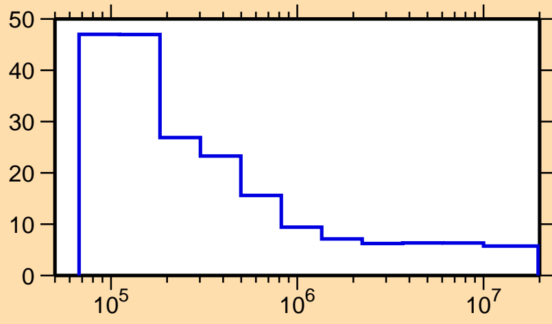
\Delta\sigma/\sigma vs. E for ^{104}\text{Tc}(n,\text{nonel.})
