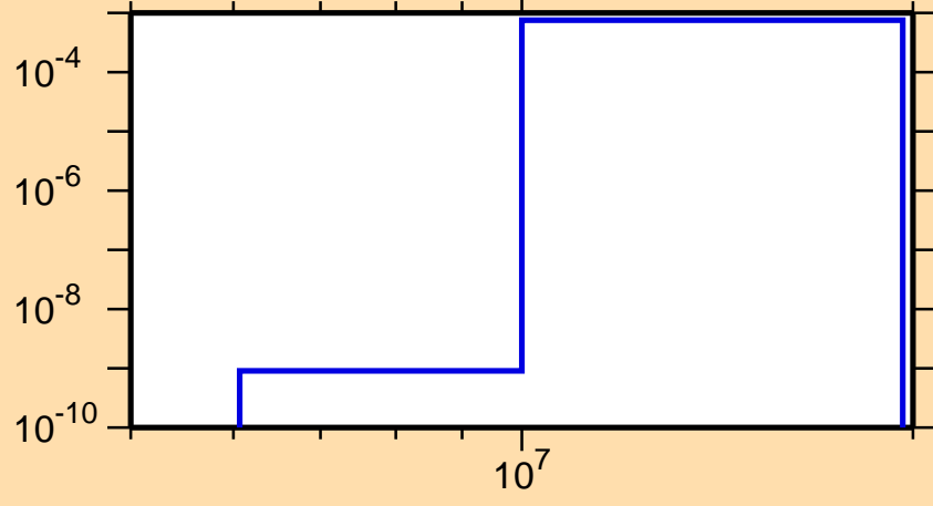
\sigma vs. E for ^{104}\text{Tc}(n,d)
