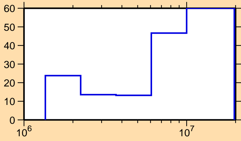
\Delta\sigma/\sigma vs. E for ^{104}\text{Tc}(n,n\text{cont.})
