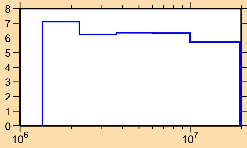
\Delta\sigma/\sigma vs. E for ^{104}\text{Tc}(n,\text{nonel.})
