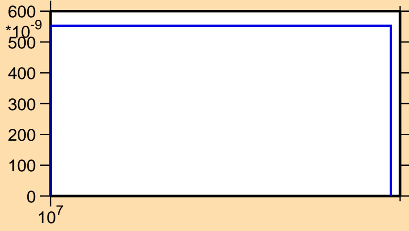
\sigma vs. E for ^{104}\text{Tc}(n,\text{nd})
