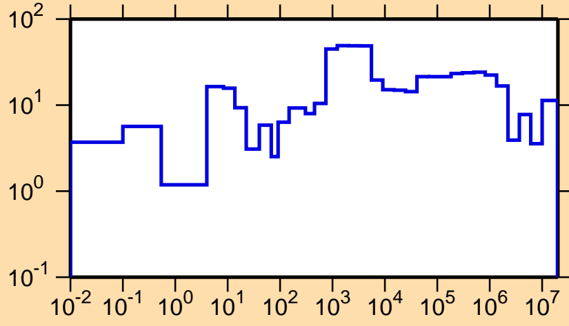
\Delta\sigma/\sigma vs. E for ^{104}\text{Tc}(n,\text{tot.})
