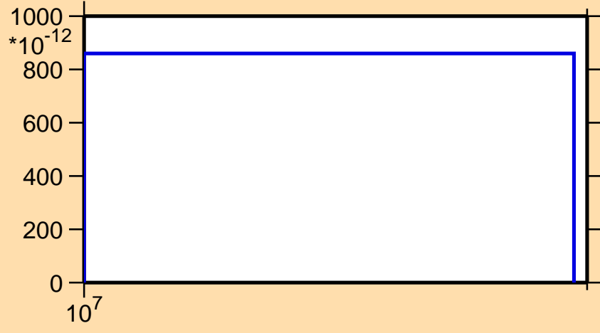
\sigma vs. E for ^{104}\text{Tc}(n,2n\alpha)
