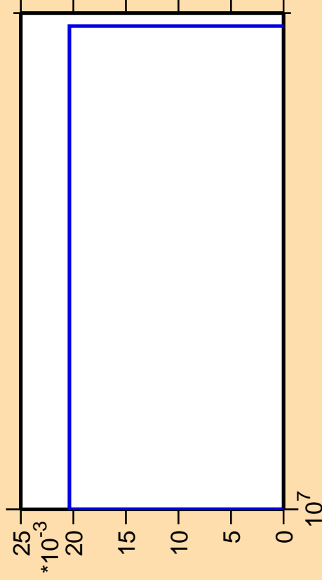
\Delta\sigma/\sigma vs. E for ^{104}\text{Tc}(n,\text{He3})
