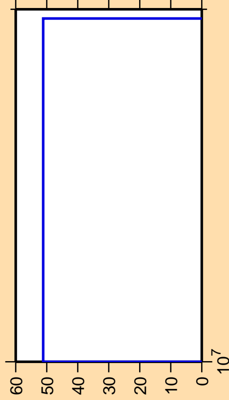
\Delta\sigma/\sigma vs. E for ^{104}\text{Tc}(n,3n)
