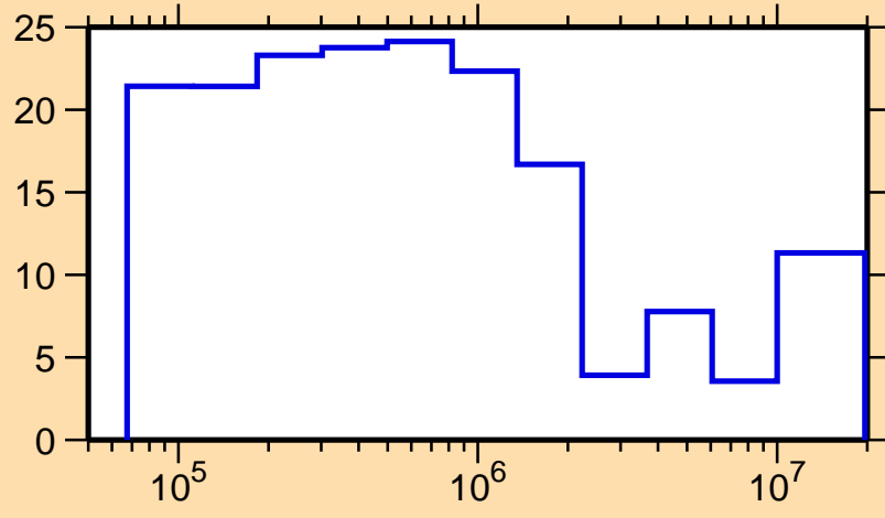
\Delta\sigma/\sigma vs. E for ^{104}\text{Tc}(n,\text{tot.})
