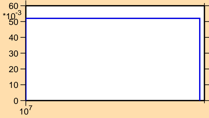
\sigma vs. E for ^{104}\text{Tc}(n,3n)
