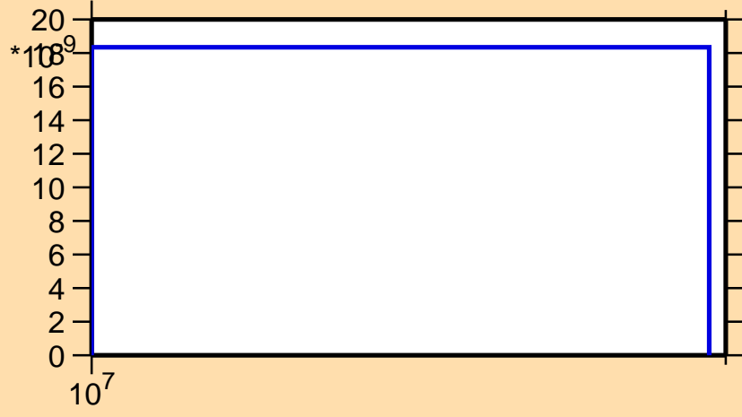
\sigma vs. E for ^{104}\text{Tc}(n,2np)
