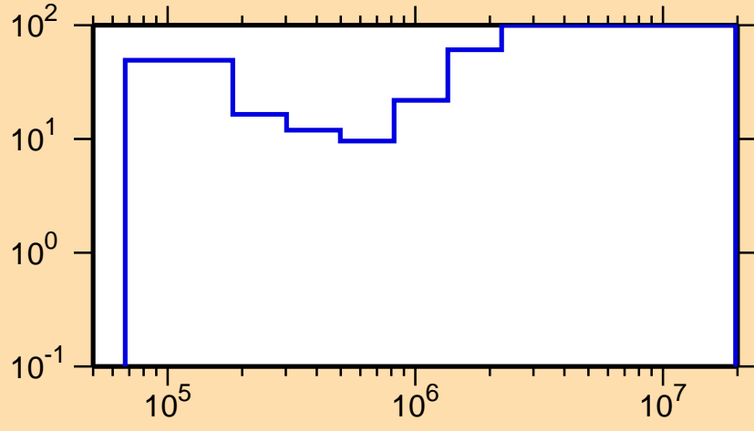
\Delta\sigma/\sigma vs. E for ^{104}\text{Tc}(n,n_1)
