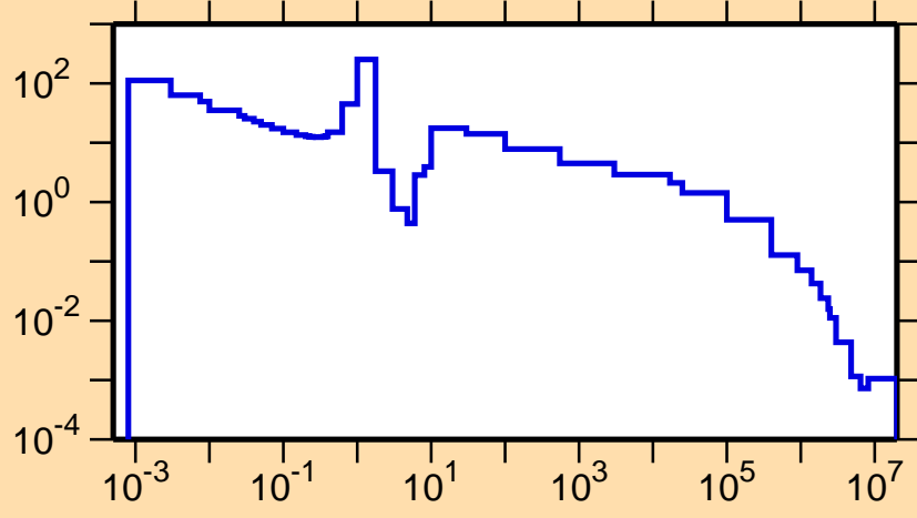
\sigma vs. E for ^{104}\text{Tc}(n,\gamma)
