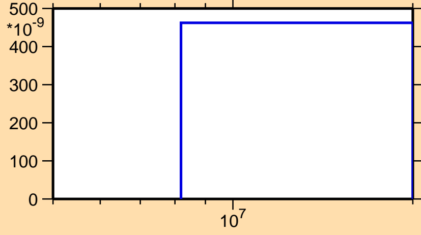
\sigma vs. E for ^{104}\text{Tc}(n,\text{nd})
