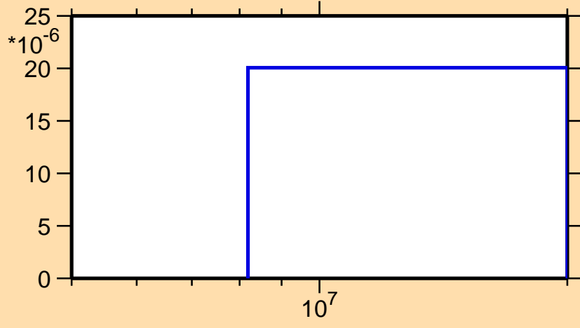
\sigma vs. E for ^{104}\text{Tc}(n,n\alpha)
