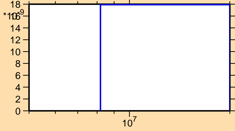
\sigma vs. E for ^{104}\text{Tc}(n,2np)
