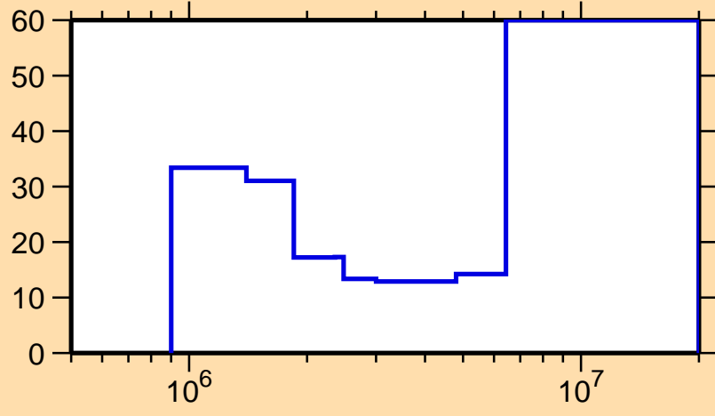
\Delta\sigma/\sigma vs. E for ^{104}\text{Tc}(n,n\text{cont.})
