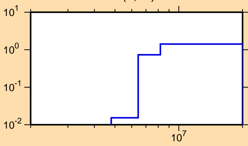
\sigma vs. E for ^{104}\text{Tc}(n,2n)
