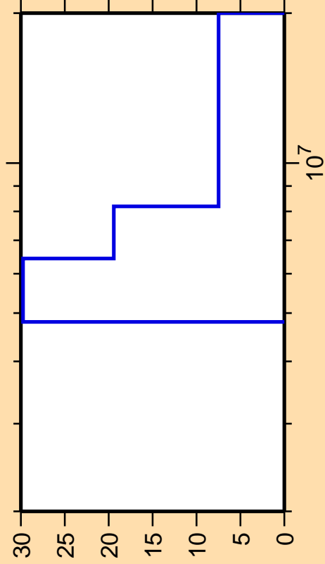
\Delta\sigma/\sigma vs. E for ^{104}\text{Tc}(n,2n)
