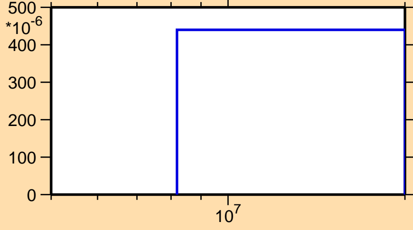
\sigma vs. E for ^{104}\text{Tc}(n,np)
