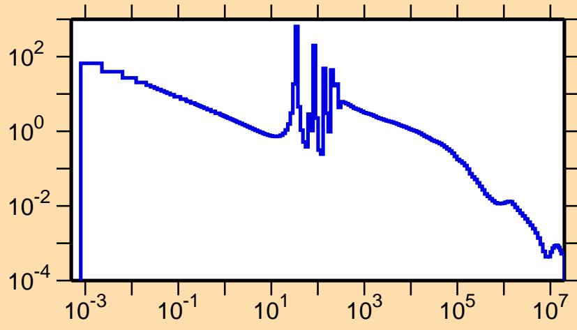
\sigma vs. E for ^{105}\text{Tc}(n,\gamma)
