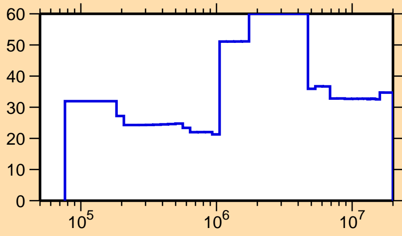
\Delta\sigma/\sigma vs. E for ^{105}\text{Tc}(n,n_1)
