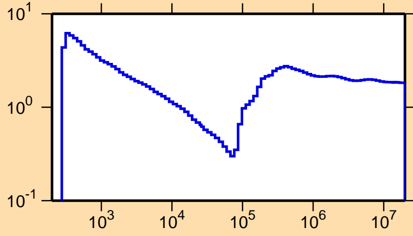
\sigma vs. E for ^{105}\text{Tc}(n,\text{nonel.})
