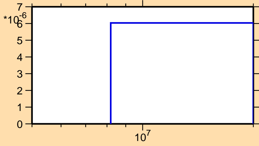
\sigma vs. E for ^{105}\text{Tc}(n,n\alpha)
