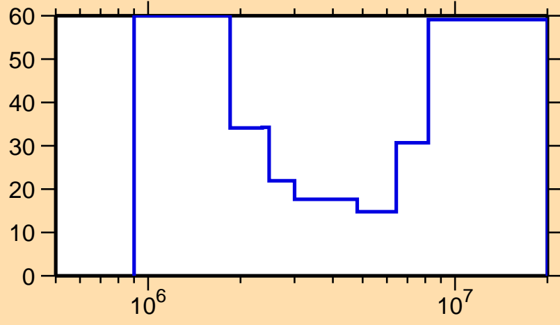
\Delta\sigma/\sigma vs. E for ^{105}\text{Tc}(n,n\text{cont.})
