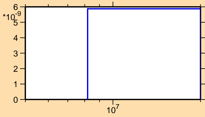
\sigma vs. E for ^{105}\text{Tc}(n,nt)
