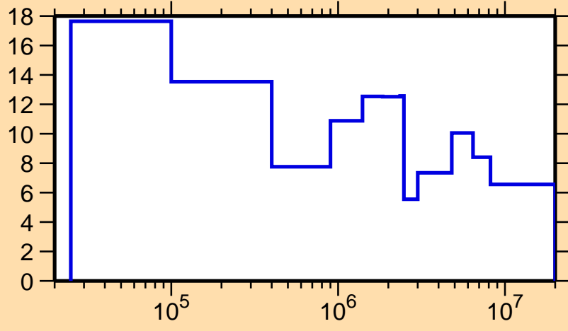
\Delta\sigma/\sigma vs. E for ^{105}\text{Tc}(n,\text{el.})
