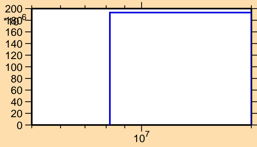
\sigma vs. E for ^{105}\text{Tc}(n,np)
