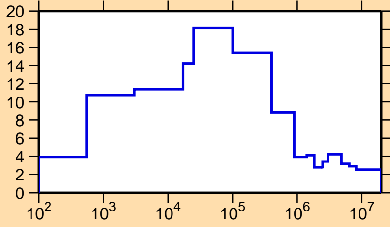
\Delta\sigma/\sigma vs. E for ^{105}\text{Tc}(n,\text{tot.})
