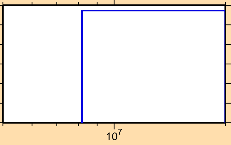
\sigma vs. E for ^{105}\text{Tc}(n,t)
