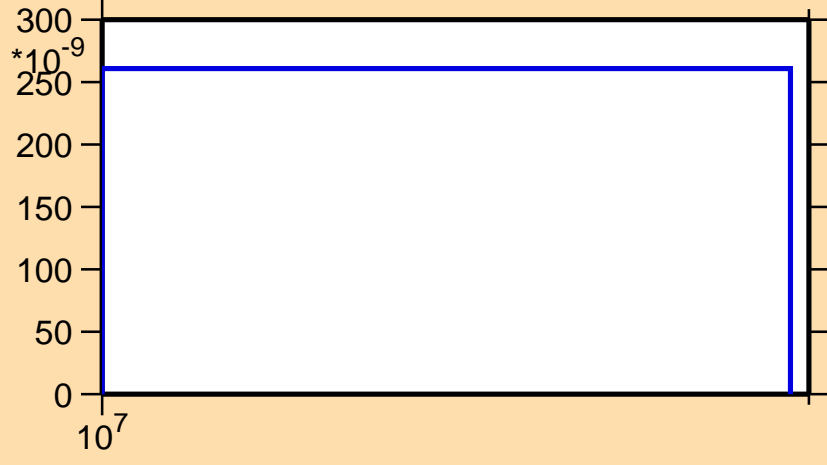
\sigma vs. E for ^{106}\text{Tc}(n,\text{nd})
