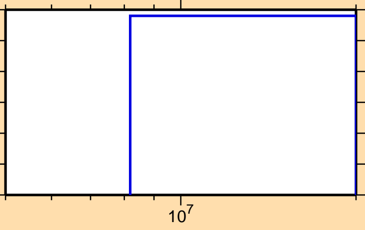
\sigma vs. E for ^{106}\text{Tc}(n,nt)
