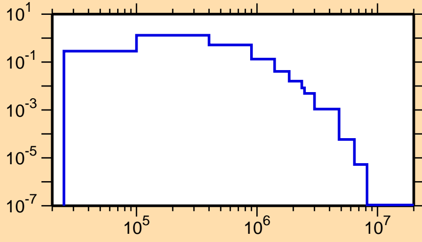
\sigma vs. E for ^{106}\text{Tc}(n,n_1)
