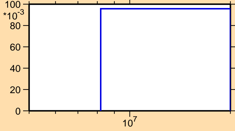
\sigma vs. E for ^{106}\text{Tc}(n,3n)
