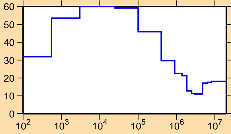
\Delta\sigma/\sigma vs. E for ^{106}\text{Tc}(n,\text{nonel.})
