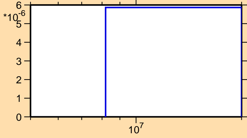
\sigma vs. E for ^{106}\text{Tc}(n,n\alpha)
