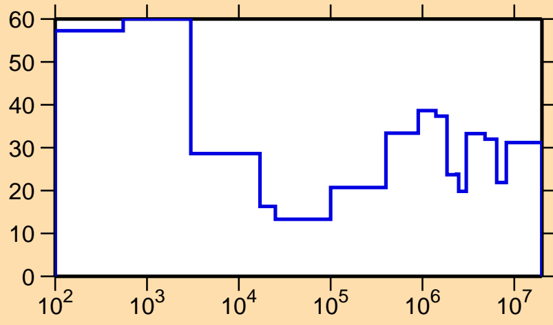
\Delta\sigma/\sigma vs. E for ^{106}\text{Tc}(n,\text{el.})
