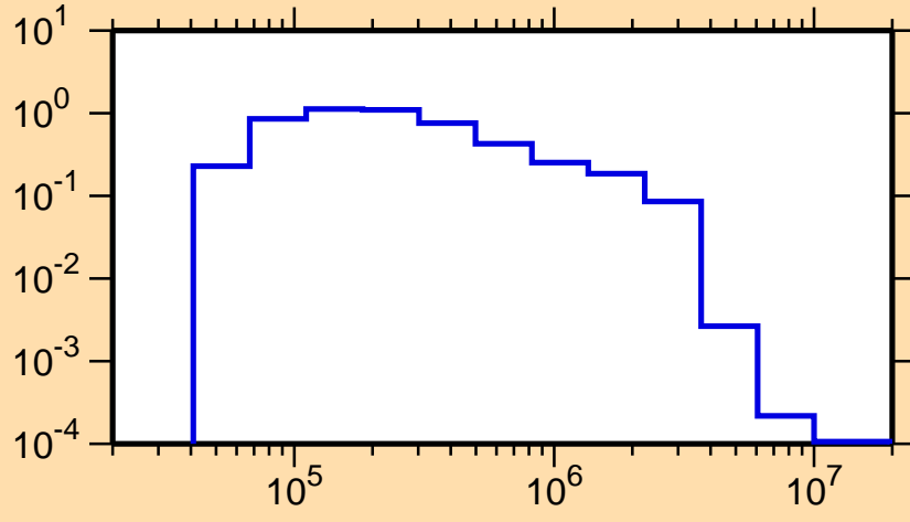
\sigma vs. E for ^{107}\text{Tc}(n,n_2)
