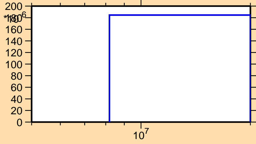
\sigma vs. E for ^{107}\text{Tc}(n,d)
