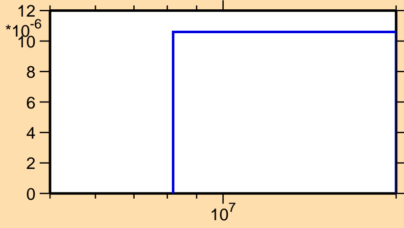
\sigma vs. E for ^{107}\text{Tc}(n,t)
