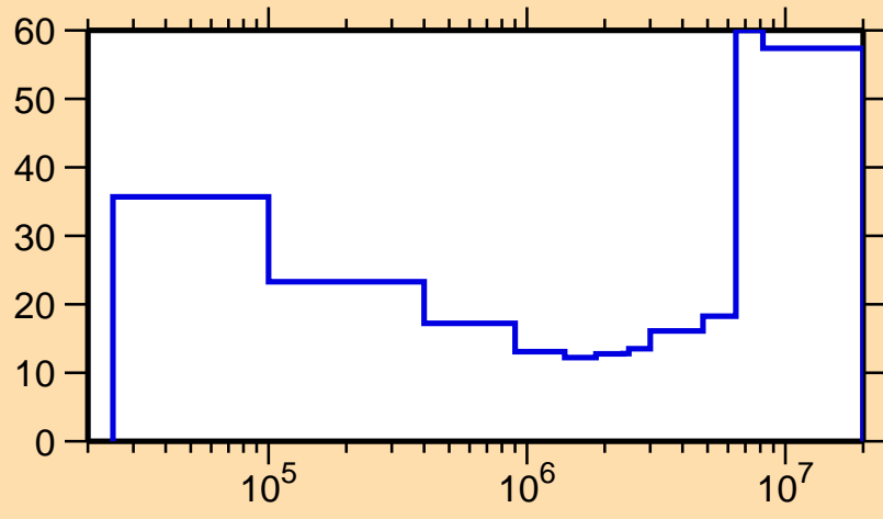
\Delta\sigma/\sigma vs. E for ^{107}\text{Tc}(n,\text{inel.})
