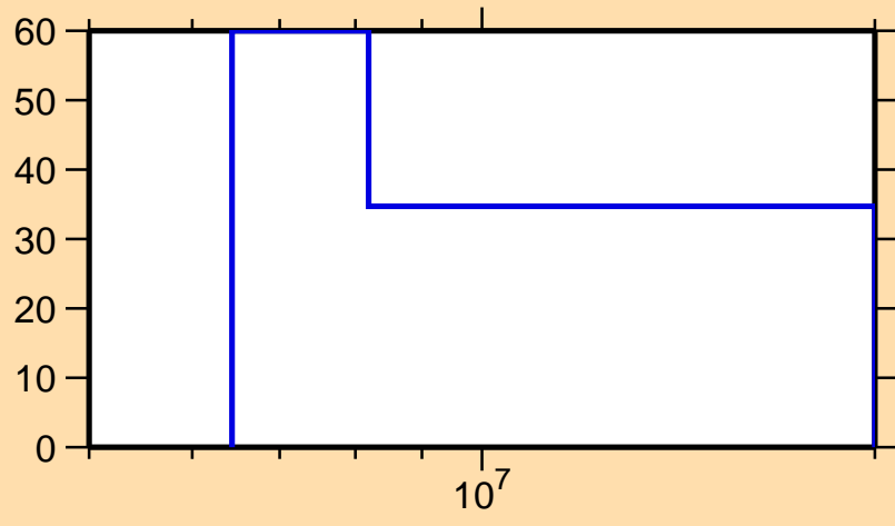
\Delta\sigma/\sigma vs. E for ^{107}\text{Tc}(n,2n)
