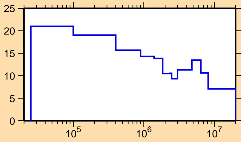
\Delta\sigma/\sigma vs. E for ^{107}\text{Tc}(n,\text{tot.})
