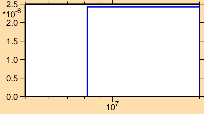
\sigma vs. E for ^{107}\text{Tc}(n,n\alpha)
