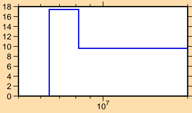
\Delta\sigma/\sigma vs. E for ^{107}\text{Tc}(n,el.)
