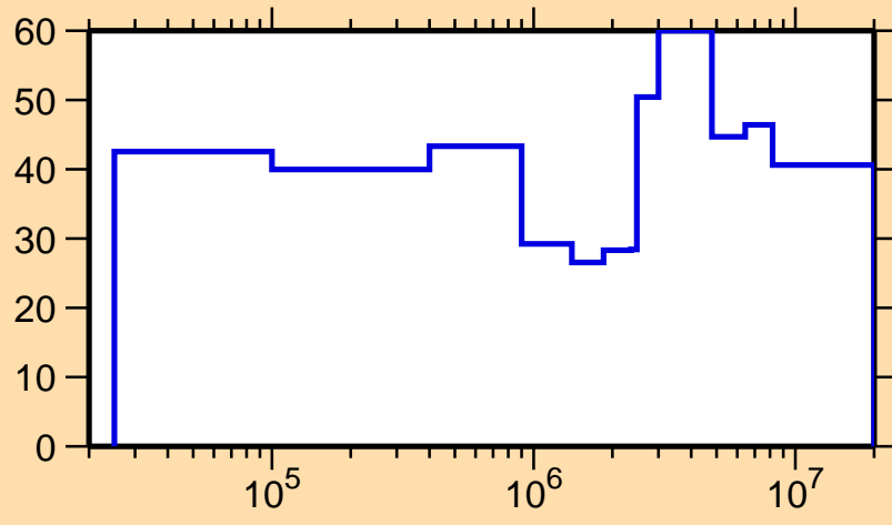
\Delta\sigma/\sigma vs. E for ^{107}\text{Tc}(n,n_1)
