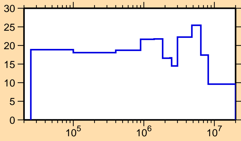
\Delta\sigma/\sigma vs. E for ^{107}\text{Tc}(n,\text{el.})
