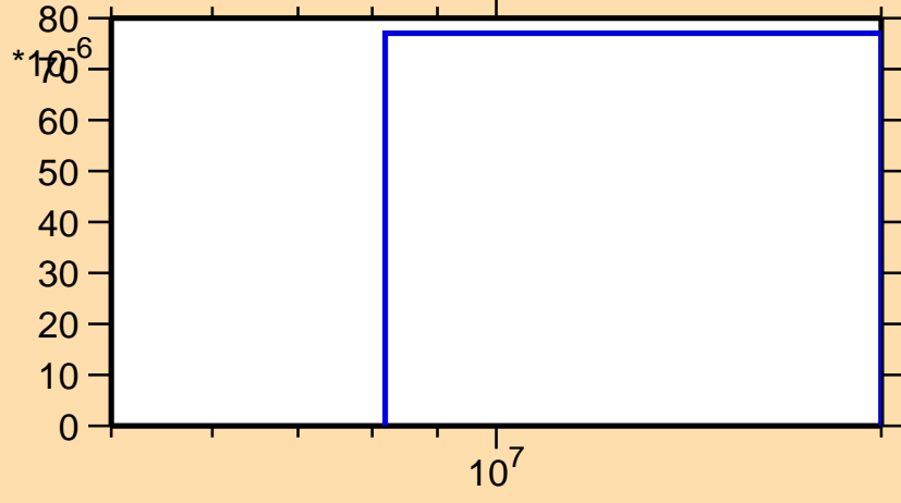
\sigma vs. E for ^{107}\text{Tc}(n,np)
