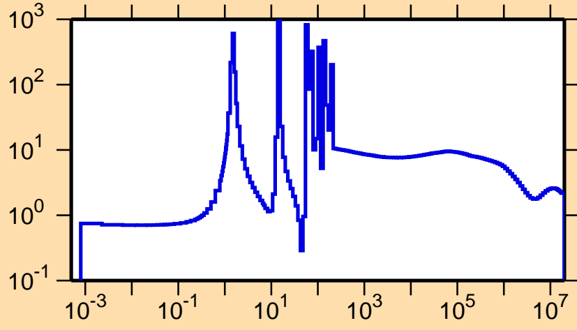
\sigma vs. E for ^{108}\text{Tc}(n,\text{el.})
