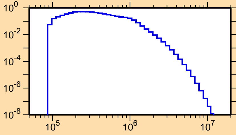
\sigma vs. E for ^{108}\text{Tc}(n,n_3)
