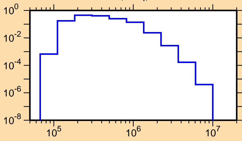
\sigma vs. E for ^{108}\text{Tc}(n,n_4)
