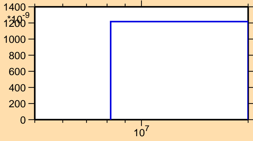
\sigma vs. E for ^{108}\text{Tc}(n,n\alpha)
