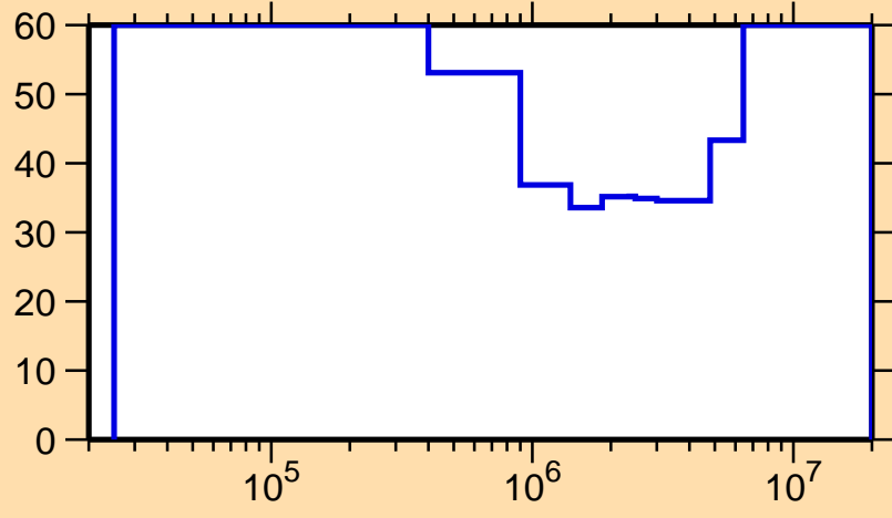
\Delta\sigma/\sigma vs. E for ^{108}\text{Tc}(n,\text{inel.})
