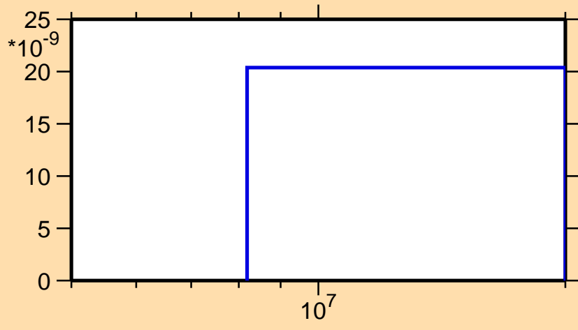
\sigma vs. E for ^{108}\text{Tc}(n,nt)
