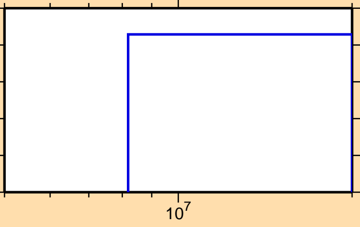
\sigma vs. E for ^{108}\text{Tc}(n,d)
