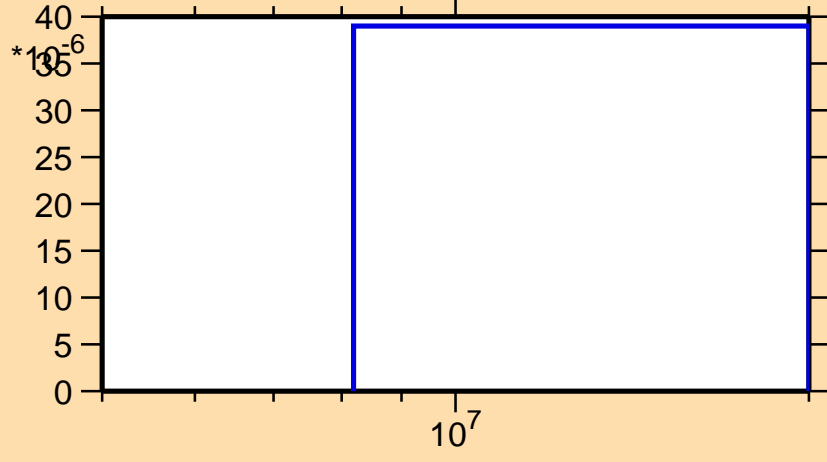
\sigma vs. E for ^{108}\text{Tc}(n,np)
