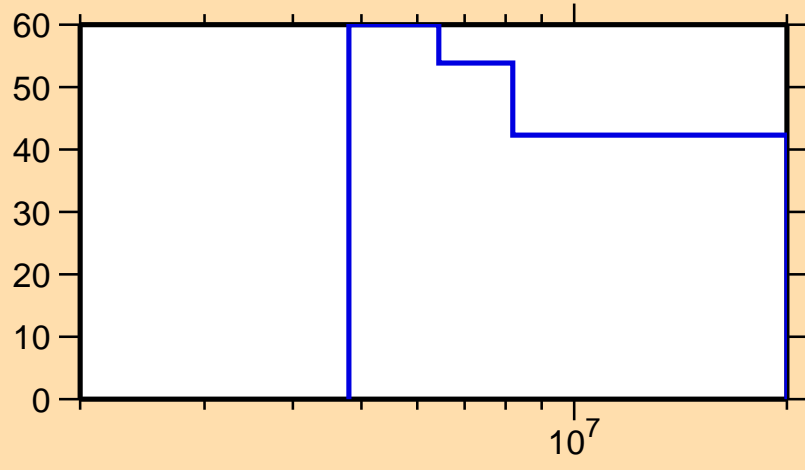
\Delta\sigma/\sigma vs. E for ^{108}\text{Tc}(n,2n)
