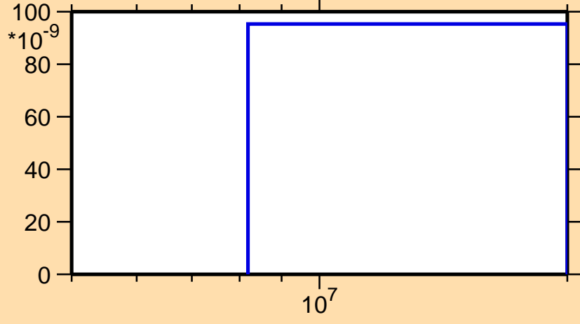
\sigma vs. E for ^{108}\text{Tc}(n,\text{nd})
