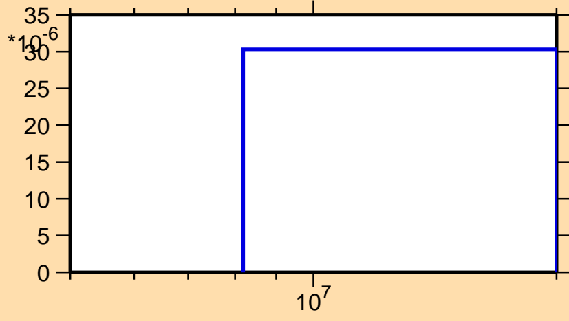
\sigma vs. E for ^{108}\text{Tc}(n,t)
