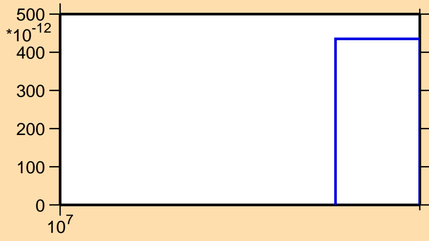
\sigma vs. E for ^{109}\text{Tc}(n,2np)
