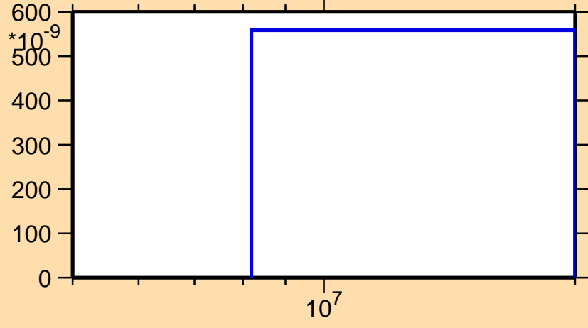
\sigma vs. E for ^{109}\text{Tc}(n,n\alpha)
