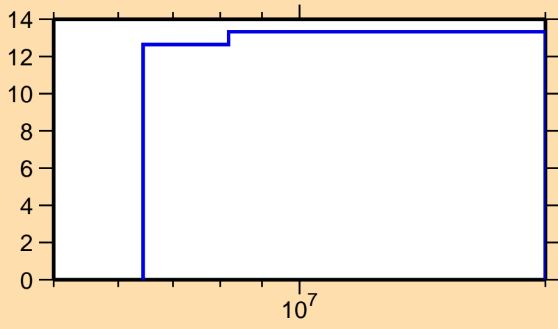
\Delta\sigma/\sigma vs. E for ^{109}\text{Tc}(n,2n)
