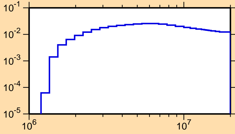
\sigma vs. E for ^{108}\text{Te}(n,n_2)
