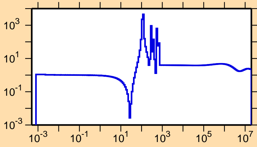
\sigma vs. E for ^{108}\text{Te}(n,\text{el.})
