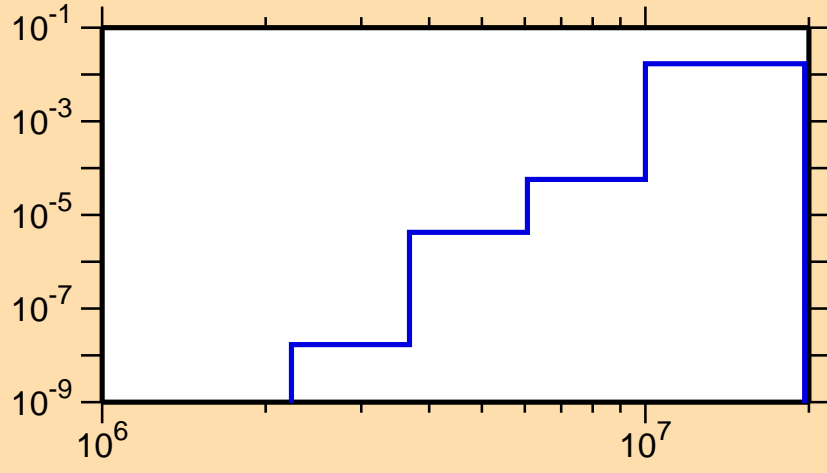
\sigma vs. E for ^{108}\text{Te}(n,d)
