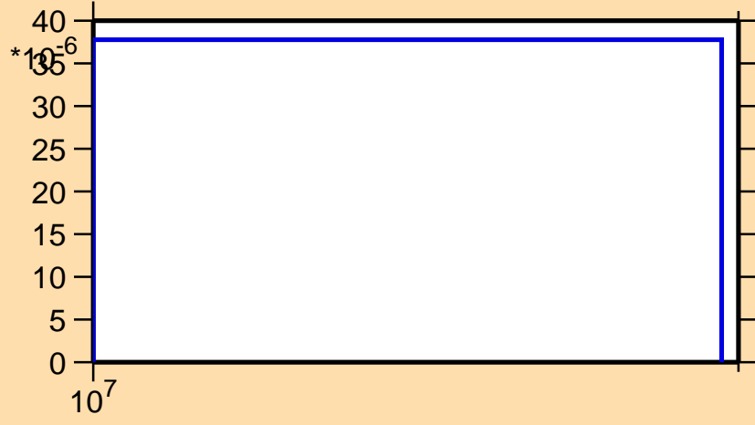
\sigma vs. E for ^{108}\text{Te}(n,2n)
