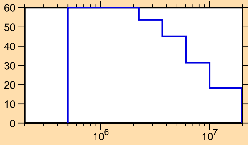
\Delta\sigma/\sigma vs. E for ^{108}\text{Te}(n,\text{inel.})
