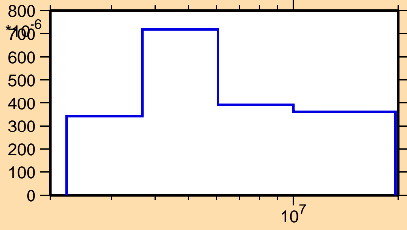
\sigma vs. E for ^{108}\text{Te}(n,n_4)
