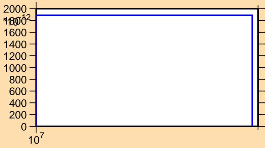
\sigma vs. E for ^{108}\text{Te}(n,\text{nd})
