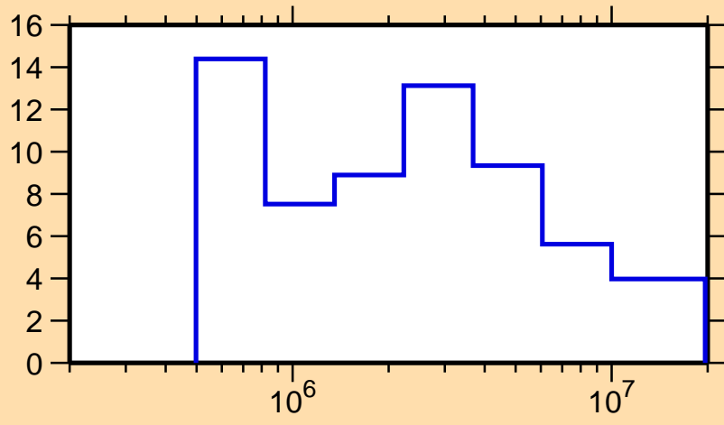
\Delta\sigma/\sigma vs. E for ^{108}\text{Te}(n,\text{el.})
