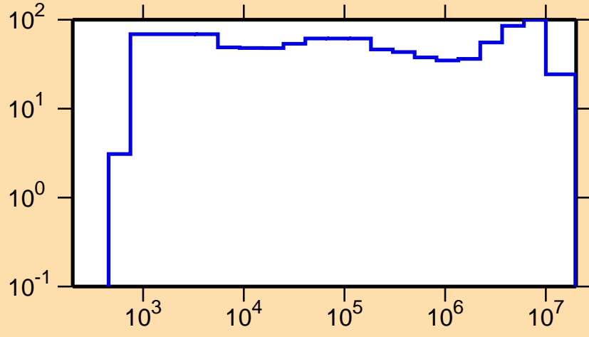
\Delta\sigma/\sigma vs. E for ^{108}\text{Te}(n,p)
