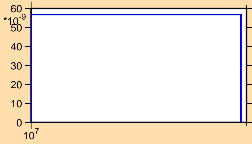
\sigma vs. E for ^{108}\text{Te}(n,2np)
