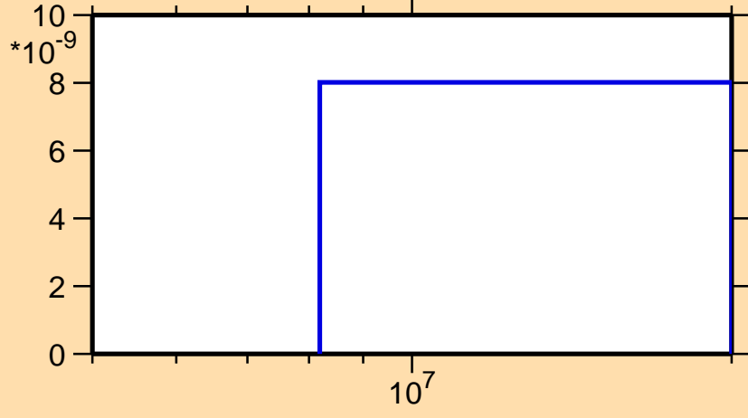
\sigma vs. E for ^{108}\text{Te} (mt 34)
