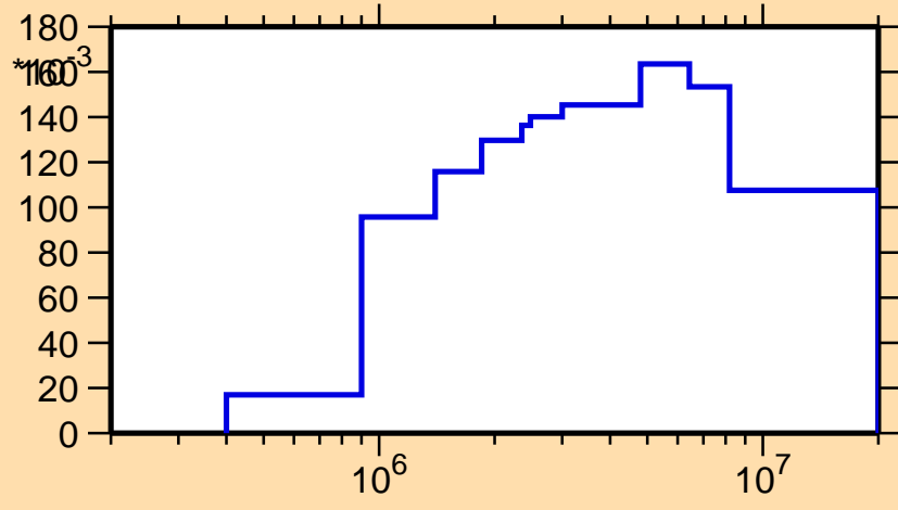
\sigma vs. E for ^{108}\text{Te}(n,\text{inel.})
