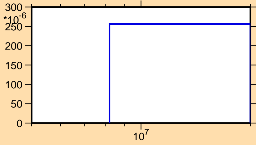
\sigma vs. E for ^{108}\text{Te}(n,t)
