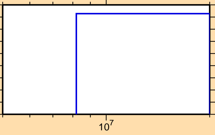
\sigma vs. E for ^{108}\text{Te}(n,\text{nd})
