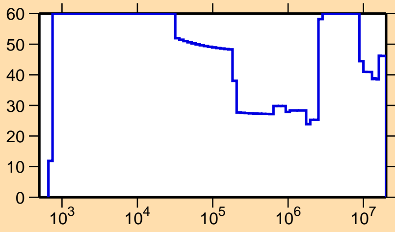
\Delta\sigma/\sigma vs. E for ^{109}\text{Te}(n,el.)
