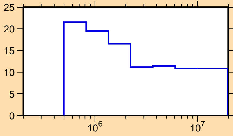
\Delta\sigma/\sigma vs. E for ^{109}\text{Te}(n,\text{nonel.})
