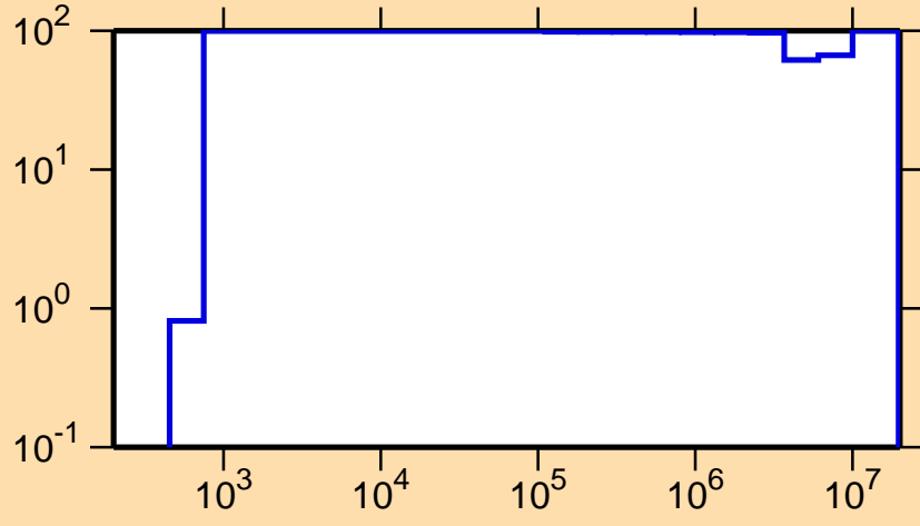
\Delta\sigma/\sigma vs. E for ^{109}\text{Te}(n,\gamma)
