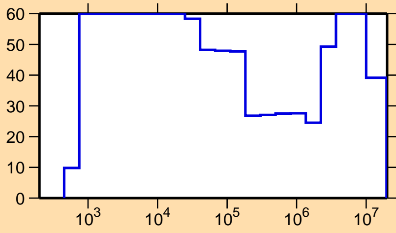
\Delta\sigma/\sigma vs. E for ^{109}\text{Te}(n,\text{el.})
