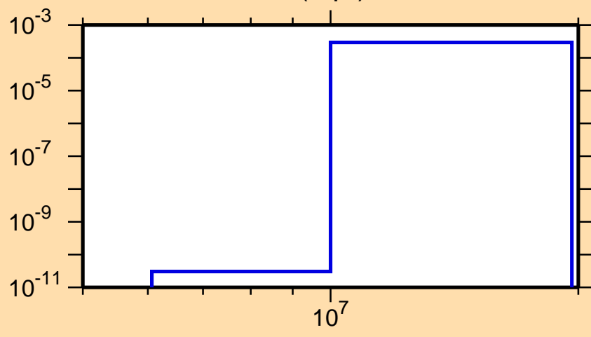
\sigma vs. E for ^{109}\text{Te}(n,\text{pt})
