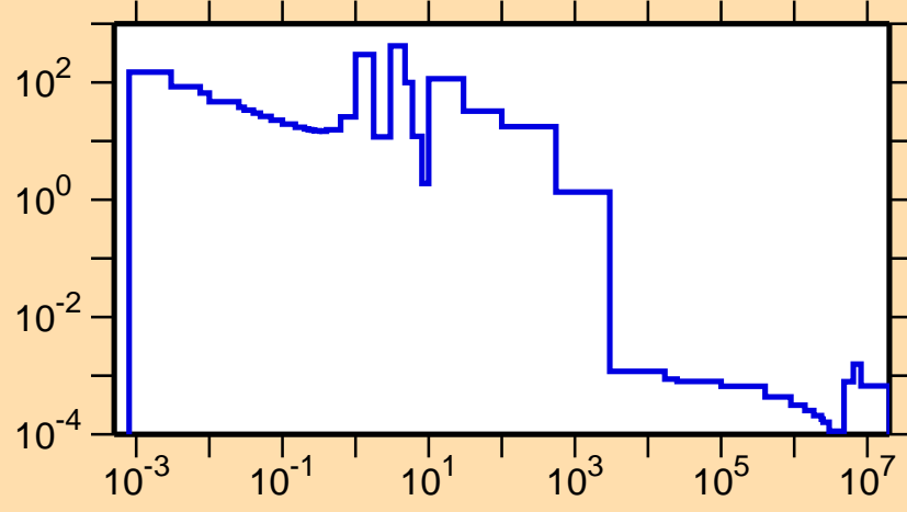
\sigma vs. E for ^{109}\text{Te}(n,\gamma)
