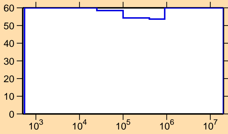
\Delta\sigma/\sigma vs. E for ^{109}\text{Te}(n,p)
