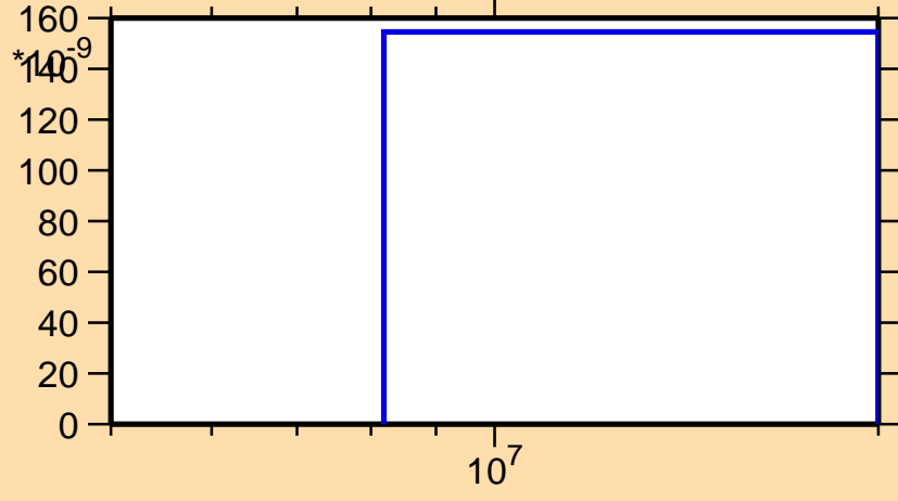
\sigma vs. E for ^{109}\text{Te}(n,nd)
