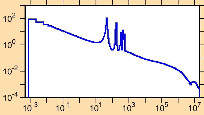
\sigma vs. E for ^{110}\text{Te}(n,\gamma)
