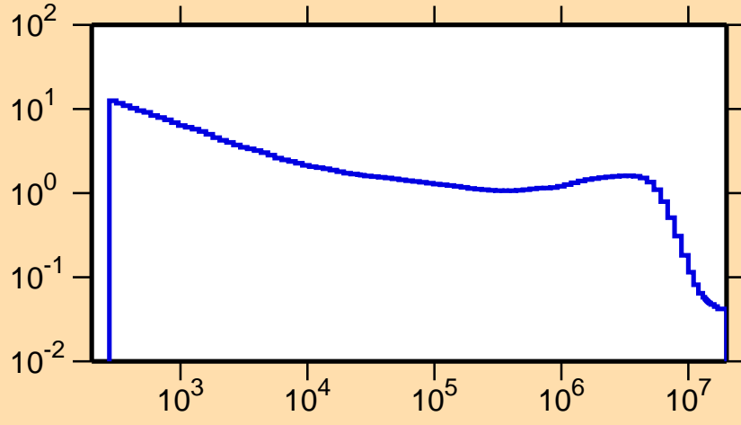
\sigma vs. E for ^{110}\text{Te}(n,p)
