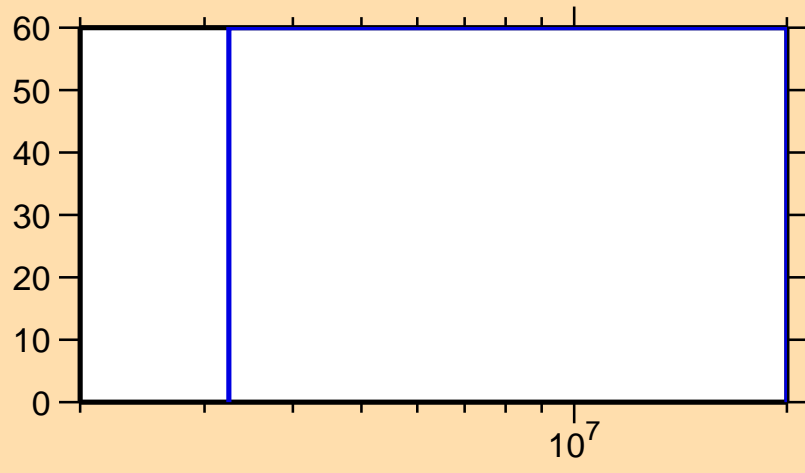
\Delta\sigma/\sigma vs. E for ^{110}\text{Te}(n,n\text{cont.})
