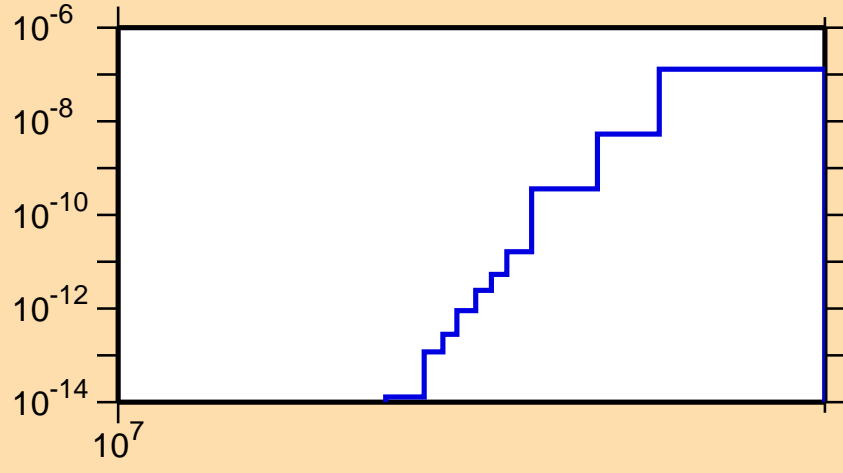
\sigma vs. E for ^{110}\text{Te}(\text{mt } 34)
