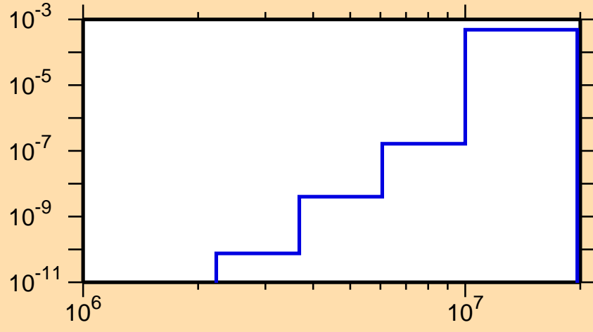
\sigma vs. E for ^{110}\text{Te}(n,\text{He}3)
