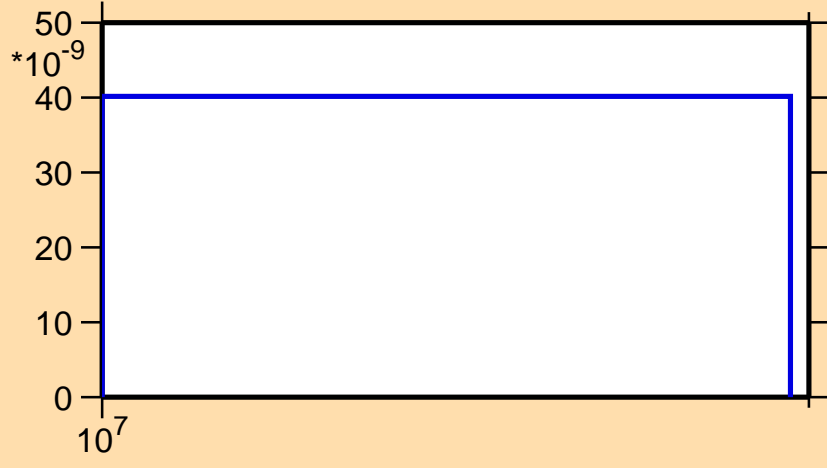
\sigma vs. E for ^{110}\text{Te}(n,2np)
