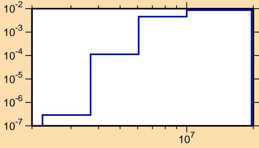
\sigma vs. E for ^{110}\text{Te}(n,n\text{cont.})
