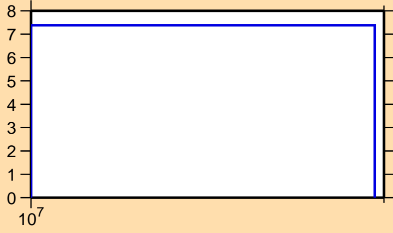
\Delta\sigma/\sigma vs. E for ^{110}\text{Te}(n,\text{nonel.})
