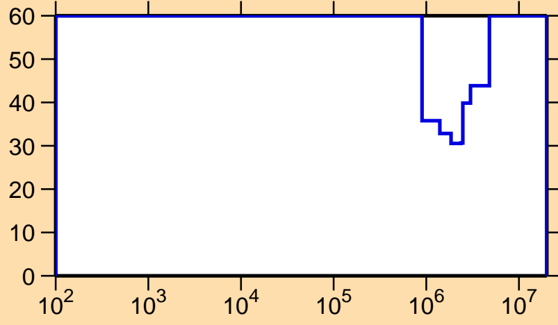
\Delta\sigma/\sigma vs. E for ^{110}\text{Te}(n,p)
