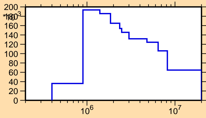
\sigma vs. E for ^{110}\text{Te}(n,n_1)
