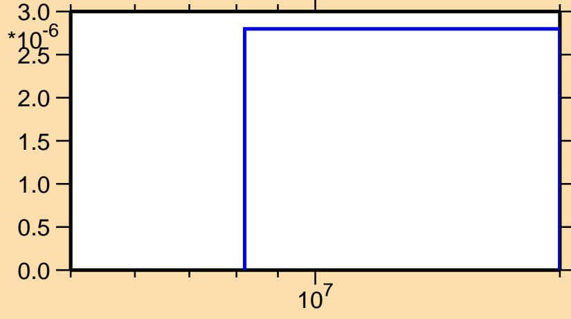
\sigma vs. E for ^{110}\text{Te}(n,\text{pt})
