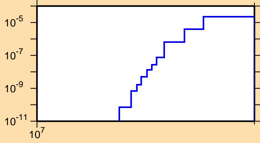
\sigma vs. E for ^{111}\text{Te}(n,\text{nd})
