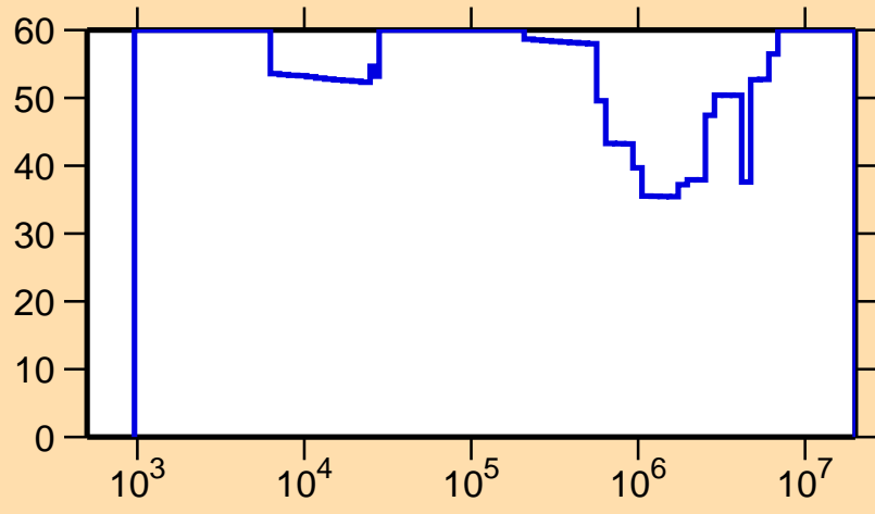
\Delta\sigma/\sigma vs. E for ^{111}\text{Te}(n,p)
