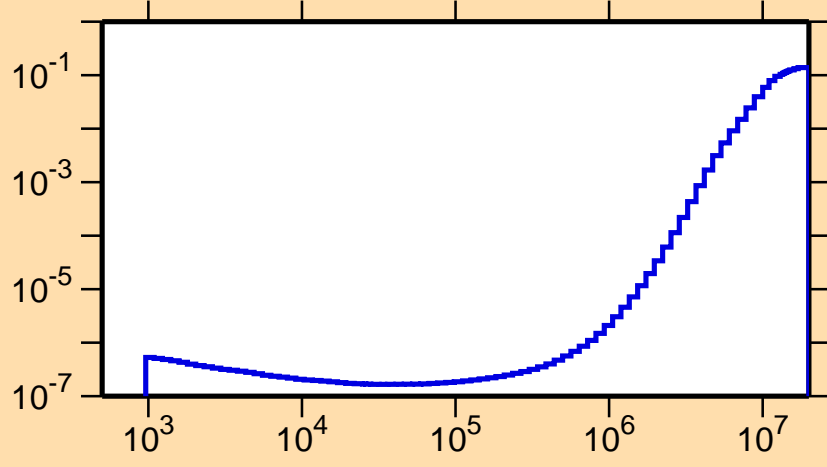
\sigma vs. E for ^{111}\text{Te}(n,p\alpha)
