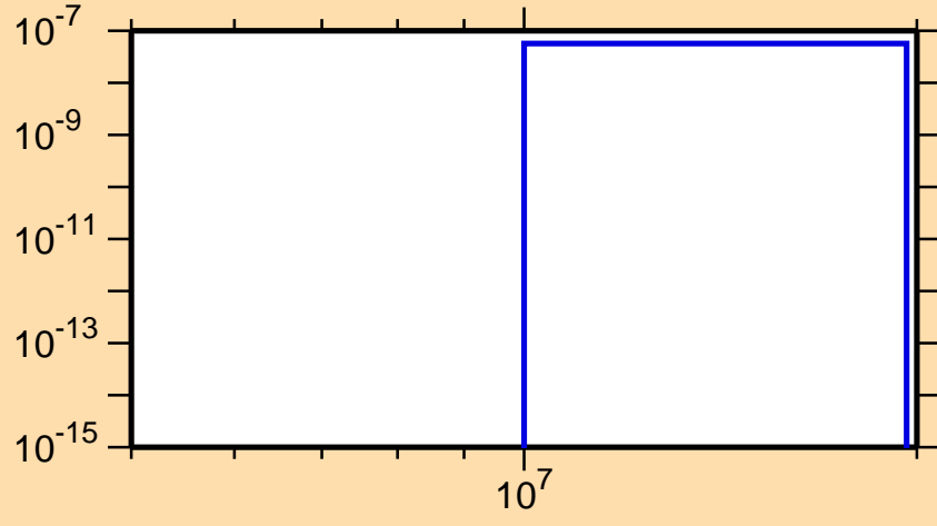
\sigma vs. E for ^{111}\text{Te}(\text{mt } 34)
