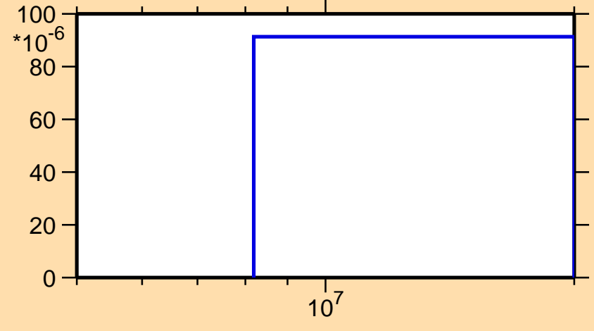
\sigma vs. E for ^{111}\text{Te}(n,2n\alpha)
