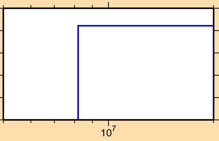
\sigma vs. E for ^{111}\text{Te}(n,\text{nd})
