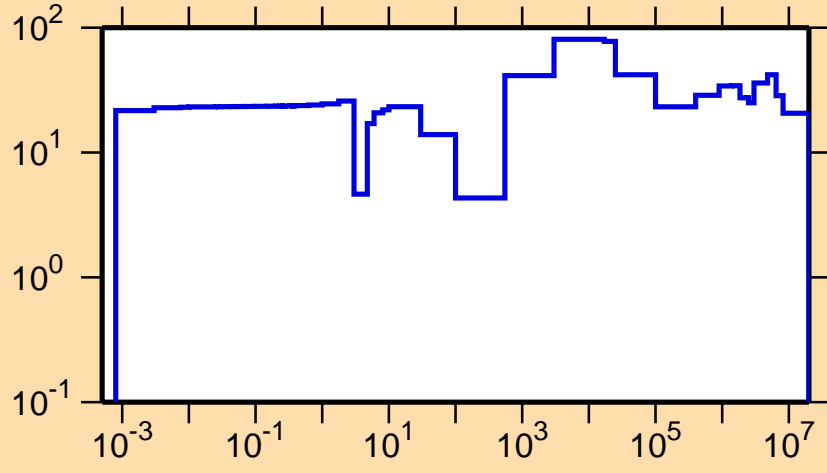
\Delta\sigma/\sigma vs. E for ^{111}\text{Te}(n,\text{el.})
