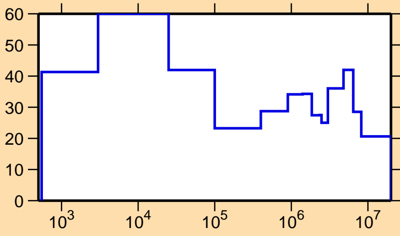
\Delta\sigma/\sigma vs. E for ^{111}\text{Te}(n,el.)
