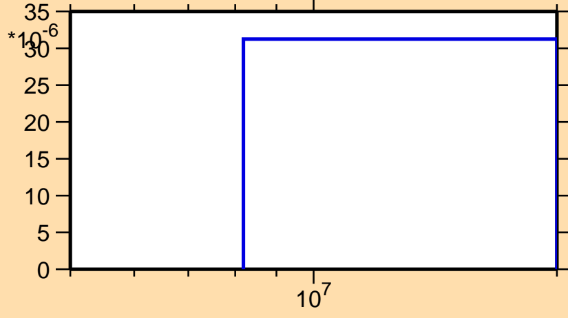
\sigma vs. E for ^{111}\text{Te}(n,\text{pt})
