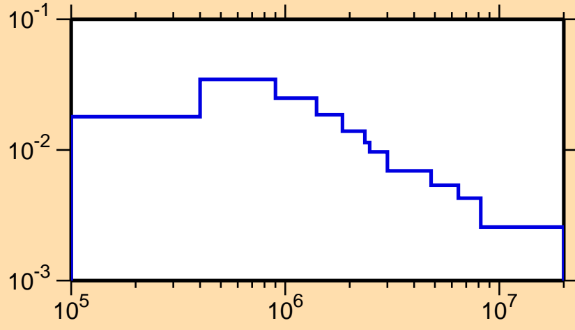
\sigma vs. E for ^{111}\text{Te}(n,n_1)
