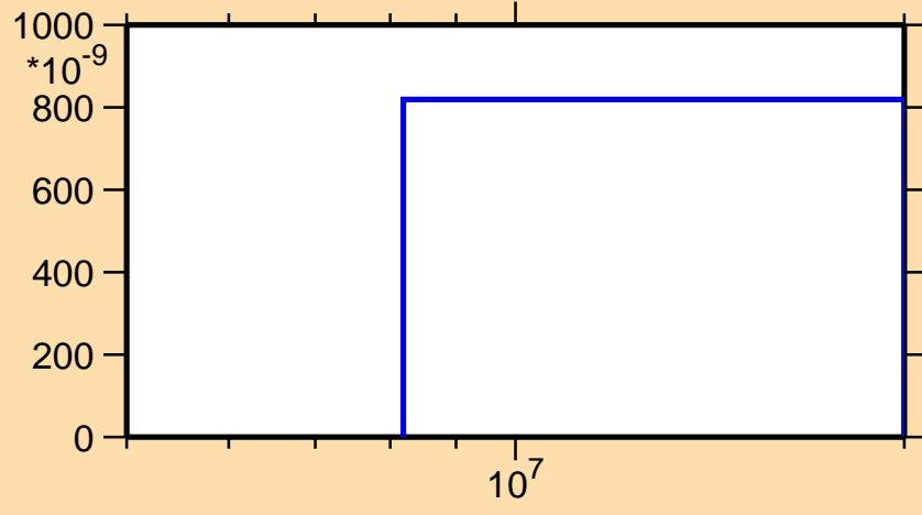
\sigma vs. E for ^{111}\text{Te}(\text{mt117})
