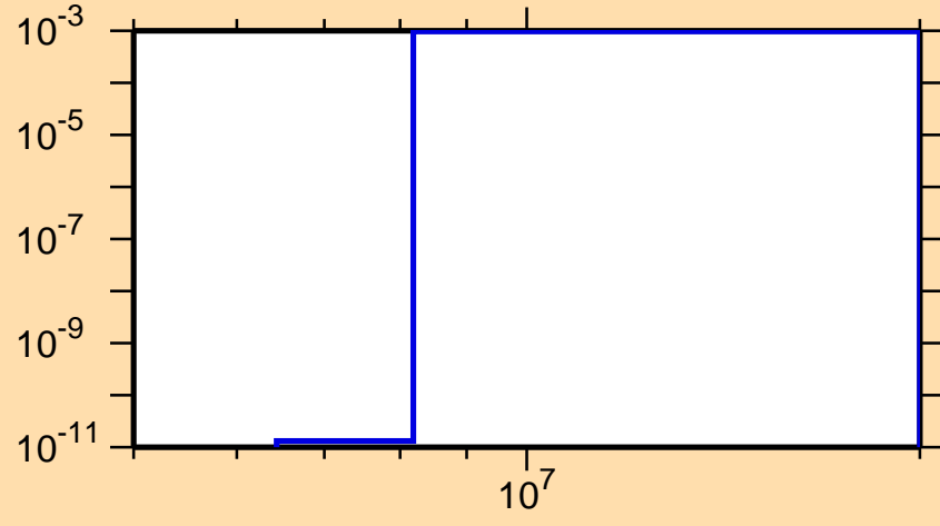
\sigma vs. E for ^{111}\text{Te}(n,pd)
