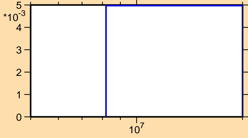
\sigma vs. E for ^{111}\text{Te}(n,2n)
