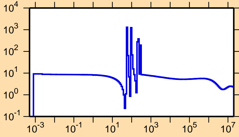
\sigma vs. E for ^{112}\text{Te}(n,\text{el.})
