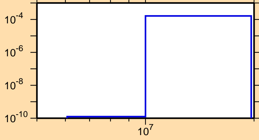
\sigma vs. E for ^{112}\text{Te}(n,pd)
