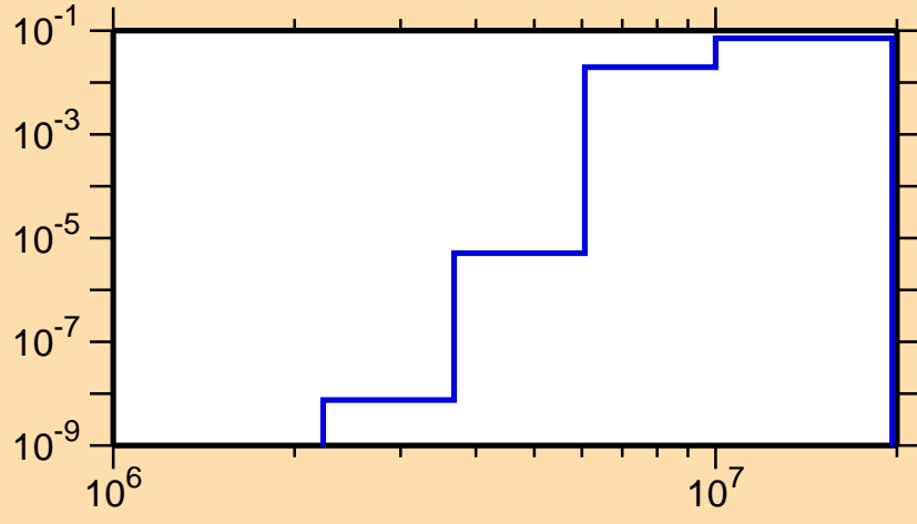
\sigma vs. E for ^{112}\text{Te}(n,n\alpha)
