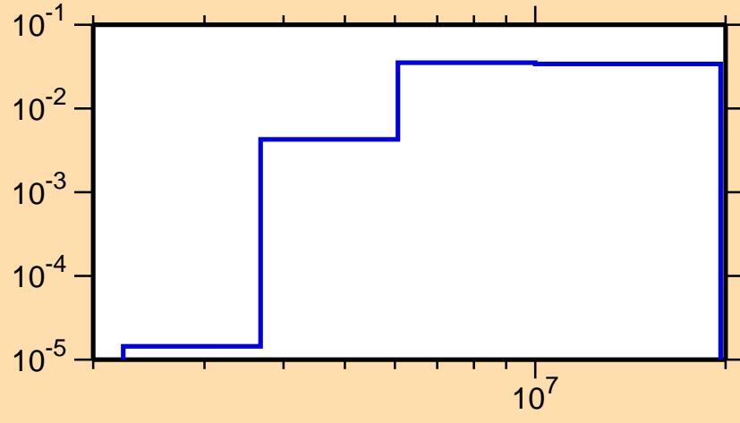
\sigma vs. E for ^{112}\text{Te}(n,n\text{cont.})
