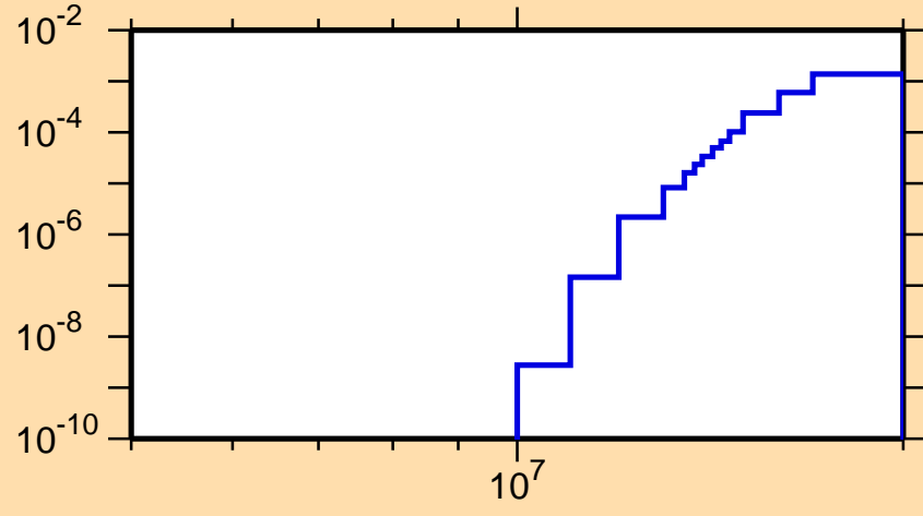
\sigma vs. E for ^{113}\text{Te}(n,pd)
