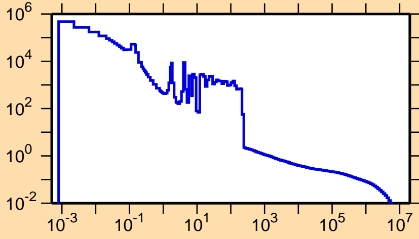
\sigma vs. E for ^{113}\text{Te}(n,\gamma)
