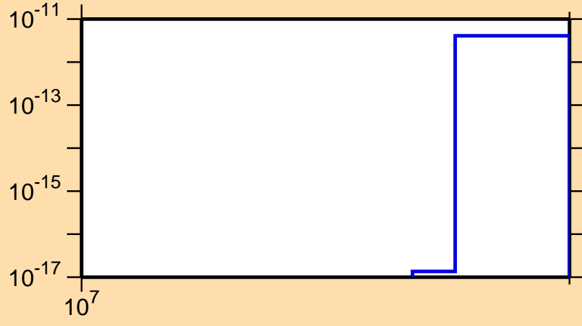
\sigma vs. E for ^{113}\text{Te}(n,nt)
