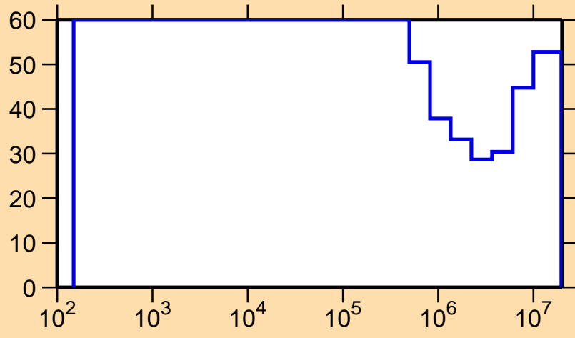
\Delta\sigma/\sigma vs. E for ^{113}\text{Te}(n,p)
