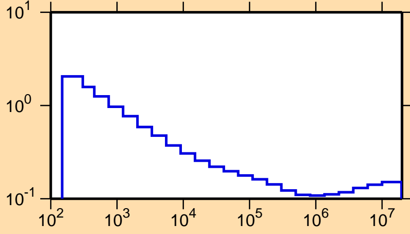
\sigma vs. E for ^{113}\text{Te}(n,\alpha)
