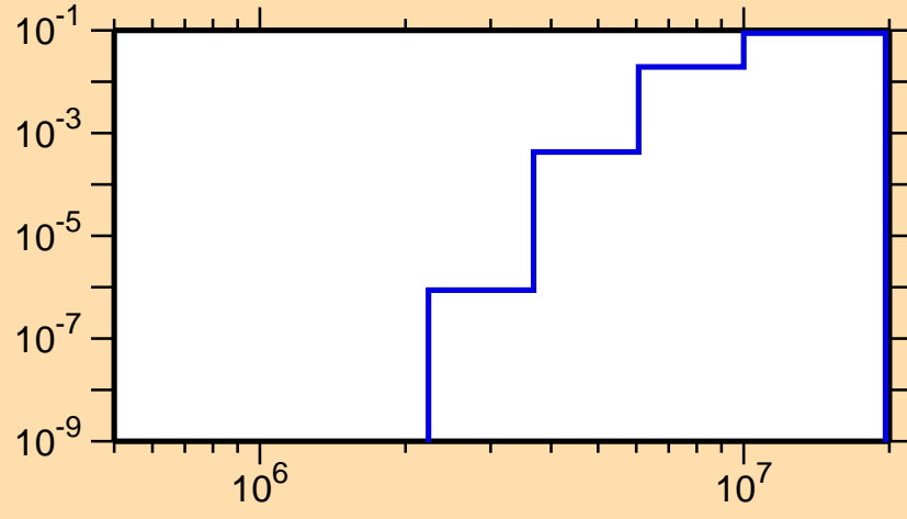
\sigma vs. E for ^{113}\text{Te}(n,n\alpha)
