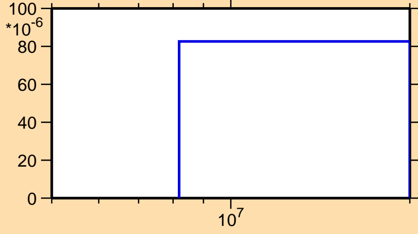
\sigma vs. E for ^{113}\text{Te}(n,pd)
