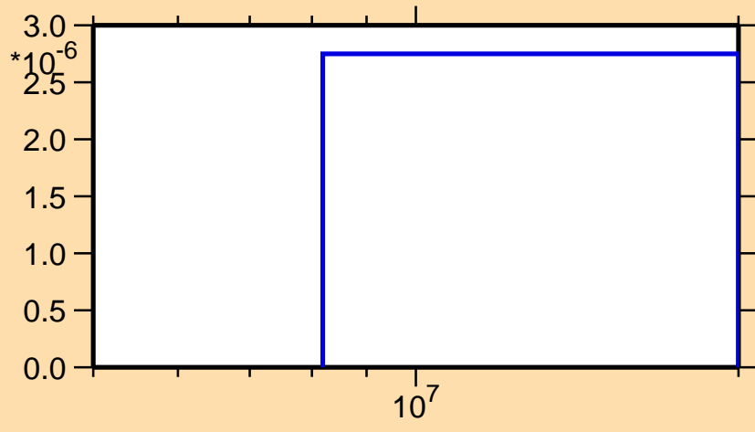
\sigma vs. E for ^{113}\text{Te}(n,\text{pt})
