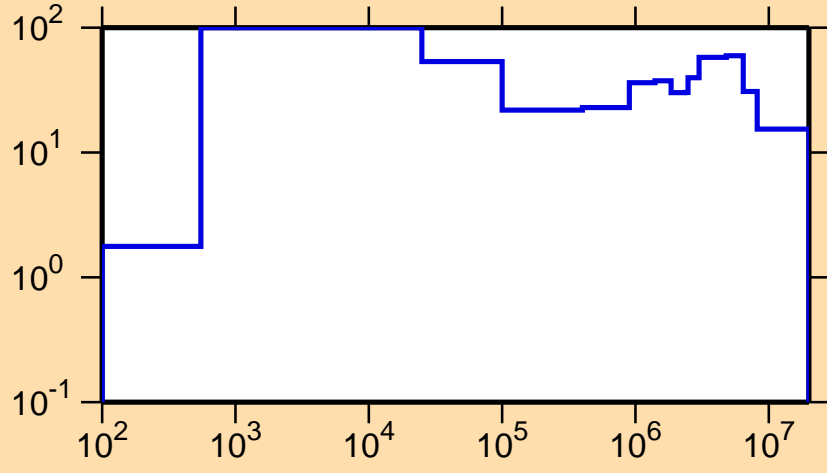
\Delta\sigma/\sigma vs. E for ^{113}\text{Te}(n,el.)
