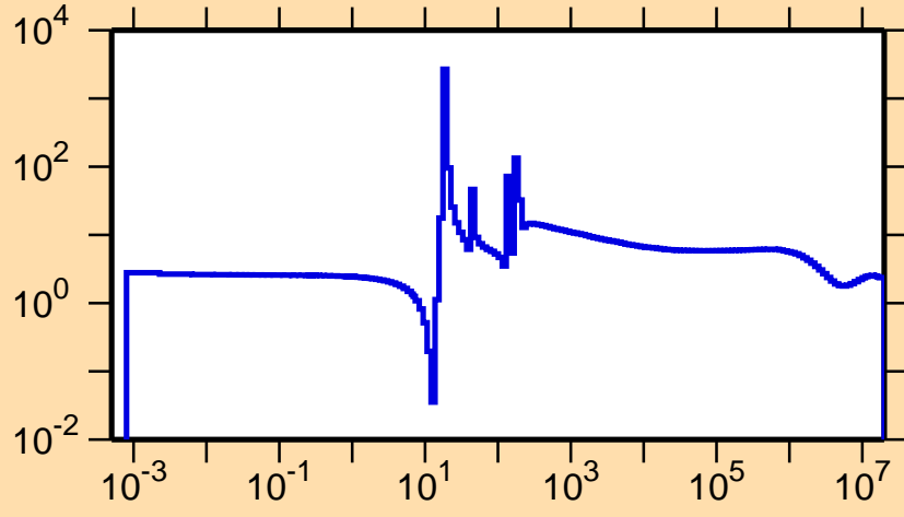
\sigma vs. E for ^{114}\text{Te}(n,\text{el.})
