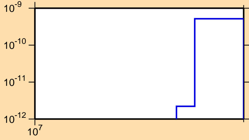
\sigma vs. E for ^{114}\text{Te} (mt 34)
