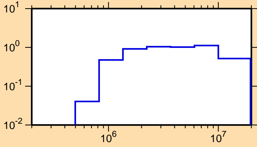
\sigma vs. E for ^{114}\text{Te}(n,\text{inel.})
