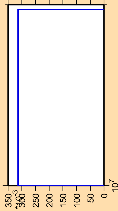
\Delta\sigma/\sigma vs. E for ^{114}\text{Te}(n,nt)
