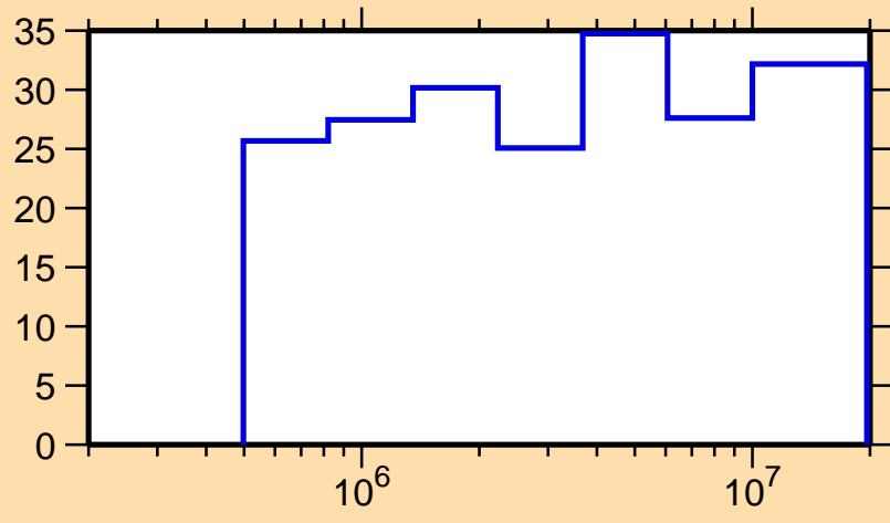
\Delta\sigma/\sigma vs. E for ^{114}\text{Te}(n,\text{el.})
