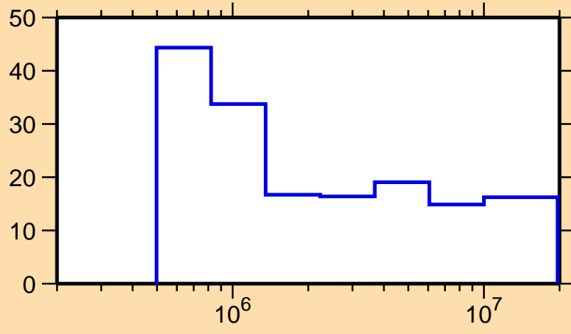
\Delta\sigma/\sigma vs. E for ^{114}\text{Te}(n,\text{nonel.})
