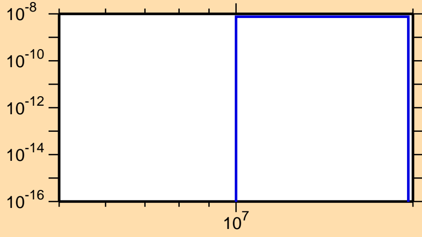
\sigma vs. E for ^{114}\text{Te}(\text{mt117})
