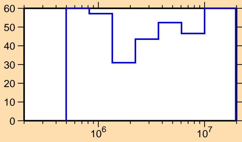
\Delta\sigma/\sigma vs. E for ^{114}\text{Te}(n,\text{inel.})
