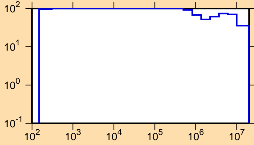
\Delta\sigma/\sigma vs. E for ^{114}\text{Te}(n,p)
