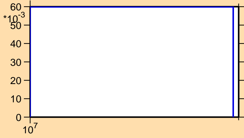
\sigma vs. E for ^{114}\text{Te}(n,2n)
