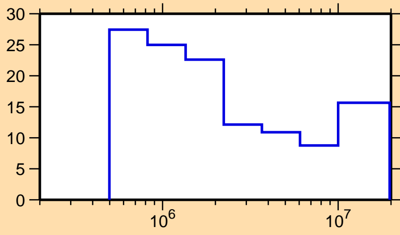
\Delta\sigma/\sigma vs. E for ^{114}\text{Te}(n,\text{tot.})
