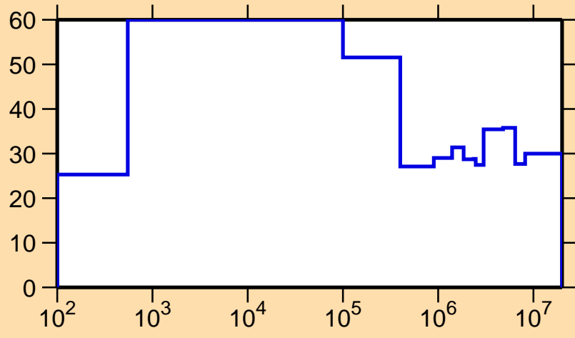
\Delta\sigma/\sigma vs. E for ^{114}\text{Te}(n,el.)
