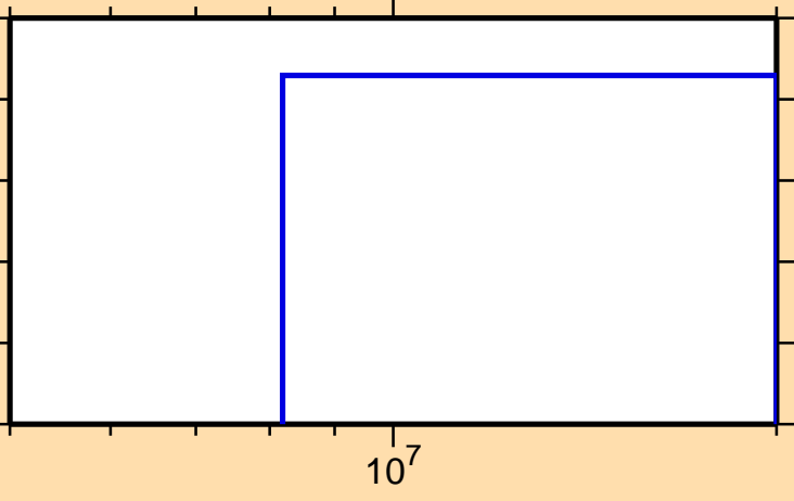
\sigma vs. E for ^{114}\text{Te}(\text{mt } 34)
