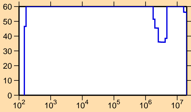
\Delta\sigma/\sigma vs. E for ^{115}\text{Te}(n,p)
