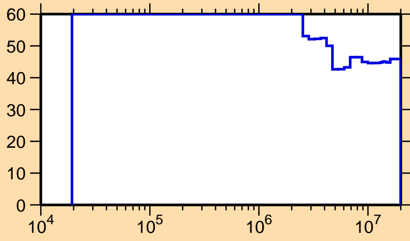
\Delta\sigma/\sigma vs. E for ^{115}\text{Te}(n,n_1)
