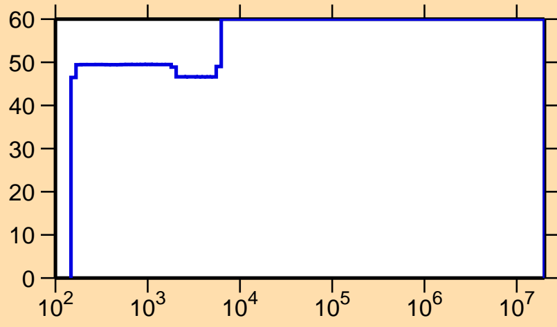
\Delta\sigma/\sigma vs. E for ^{115}\text{Te}(n,\gamma)
