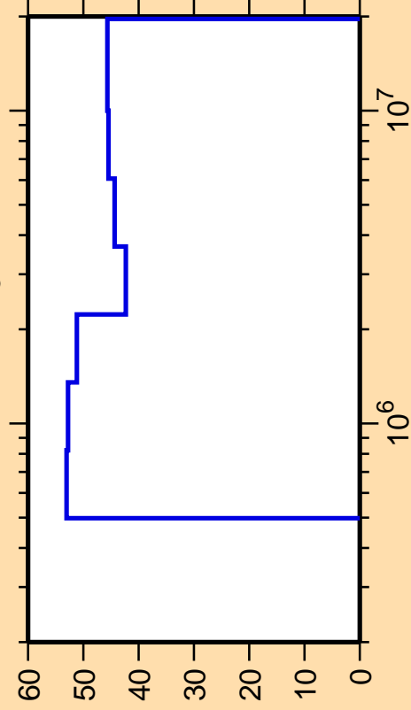
\Delta\sigma/\sigma vs. E for ^{115}\text{Te}(n,n_3)
