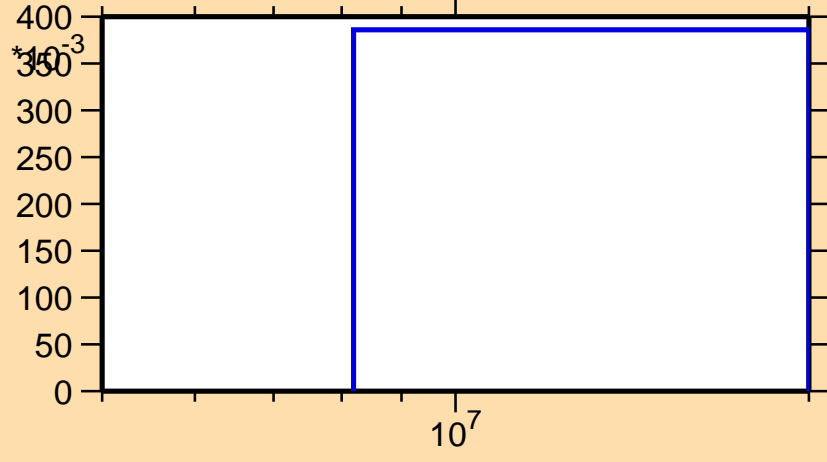
\sigma vs. E for ^{115}\text{Te}(n,2n)
