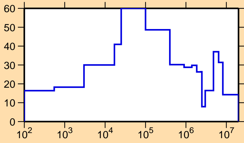
\Delta\sigma/\sigma vs. E for ^{115}\text{Te}(n,el.)
