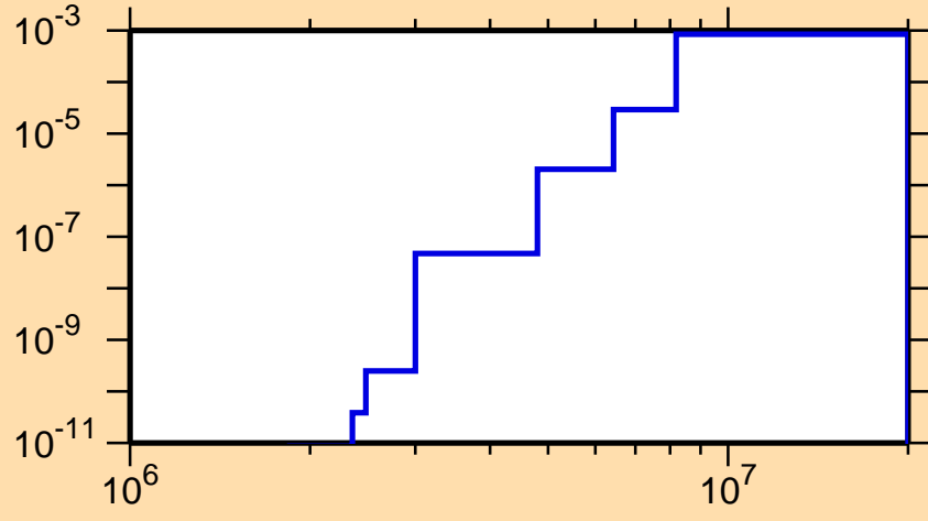
\sigma vs. E for ^{115}\text{Te}(n,p\alpha)
