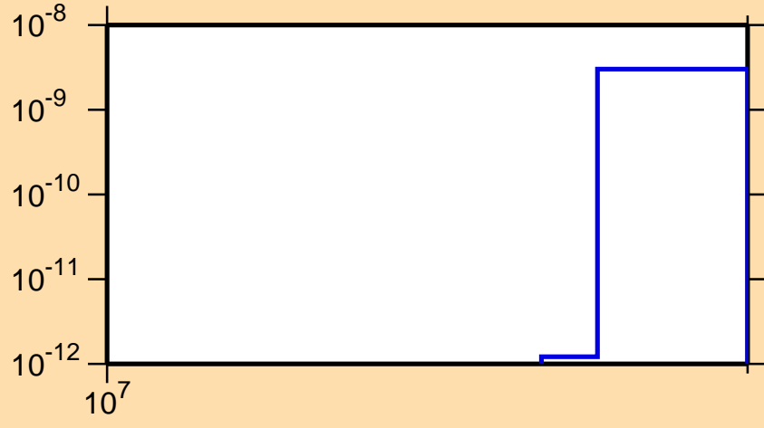
\sigma vs. E for ^{116}\text{Te}(n,\text{pt})
