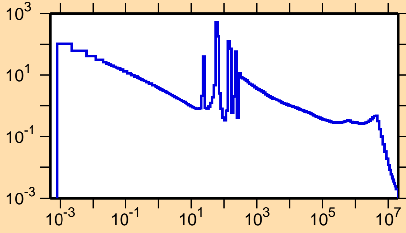
\sigma vs. E for ^{116}\text{Te}(n,\gamma)
