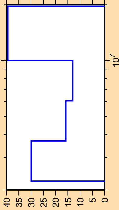
\Delta\sigma/\sigma vs. E for ^{116}\text{Te}(n,n\text{cont.})
