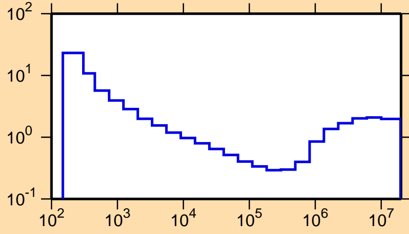
\sigma vs. E for ^{116}\text{Te}(n,\text{nonel.})
