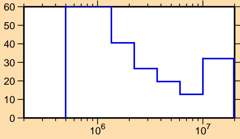
\Delta\sigma/\sigma vs. E for ^{116}\text{Te}(n,\text{inel.})
