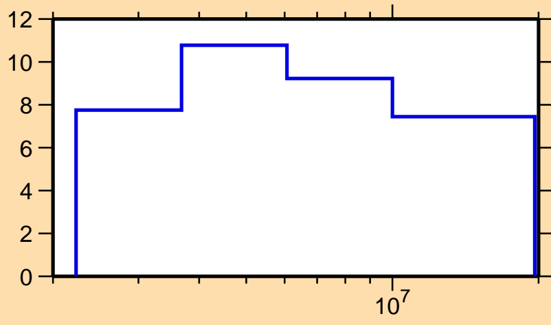
\Delta\sigma/\sigma vs. E for ^{116}\text{Te}(n,n\text{onel.})
