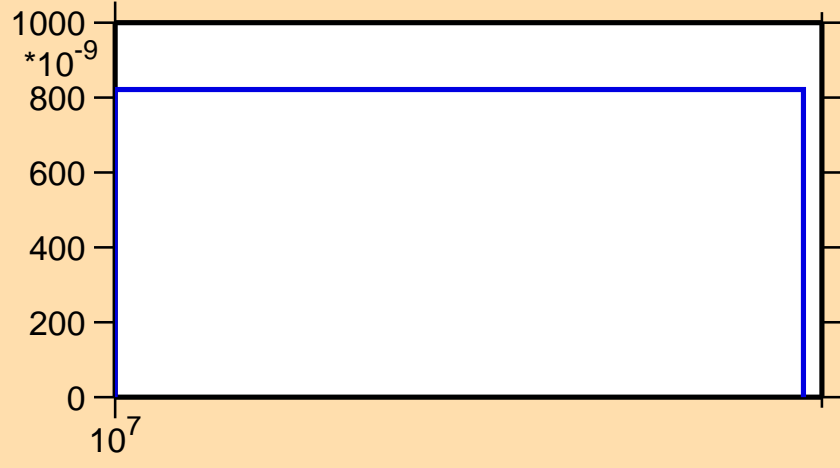
\sigma vs. E for ^{116}\text{Te}(n,2n\alpha)
