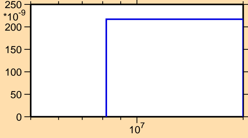
\sigma vs. E for ^{116}\text{Te}(n,pd)
