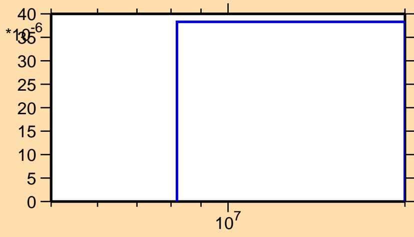
\sigma vs. E for ^{116}\text{Te}(n,t)
