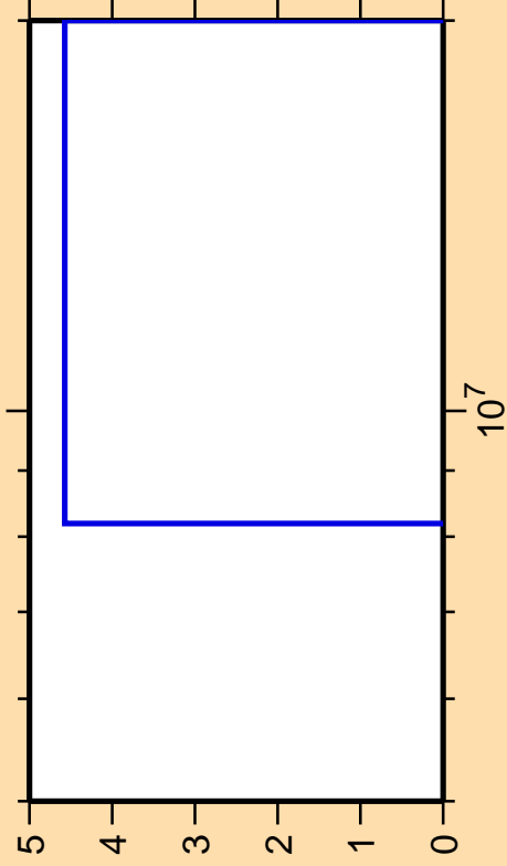
\Delta\sigma/\sigma vs. E for ^{116}\text{Te}(n,nt)
