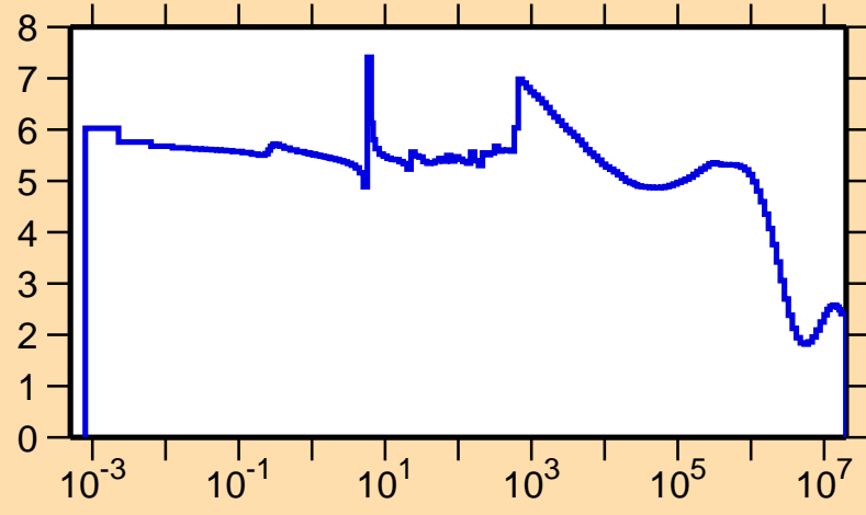
\sigma vs. E for ^{117}\text{Te}(n,\text{el.})
