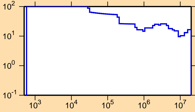
\Delta\sigma/\sigma vs. E for ^{117}\text{Te}(n,el.)
