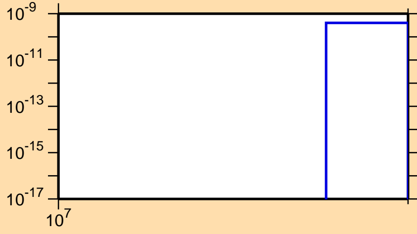
\sigma vs. E for ^{117}\text{Te}(n,nt)
