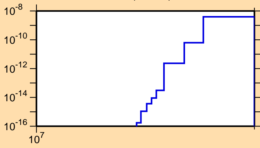
\sigma vs. E for ^{117}\text{Te} (mt 34)
