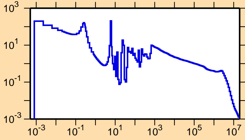
\sigma vs. E for ^{117}\text{Te}(n,\gamma)
