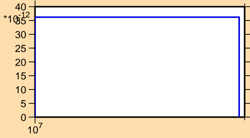
\sigma vs. E for ^{117}\text{Te} (mt 34)
