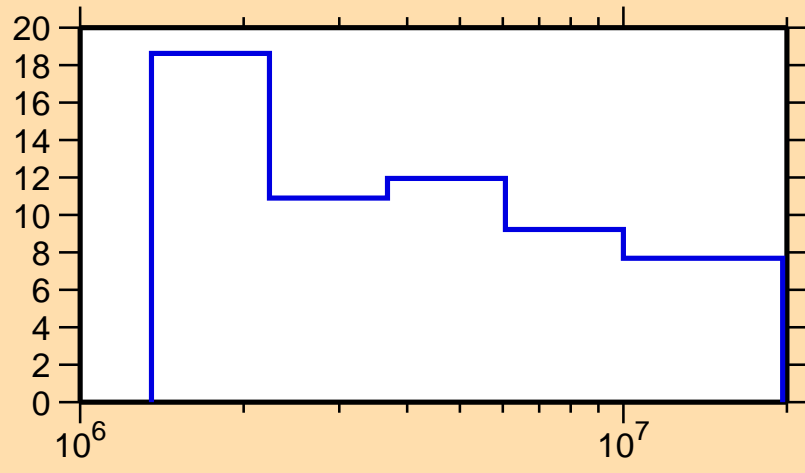
\Delta\sigma/\sigma vs. E for ^{117}\text{Te}(n,\text{nonel.})
