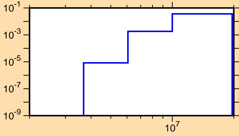
\sigma vs. E for ^{117}\text{Te}(n,n\alpha)
