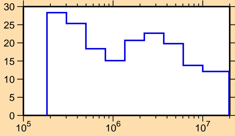
\Delta\sigma/\sigma vs. E for ^{117}\text{Te}(n,\text{el.})
