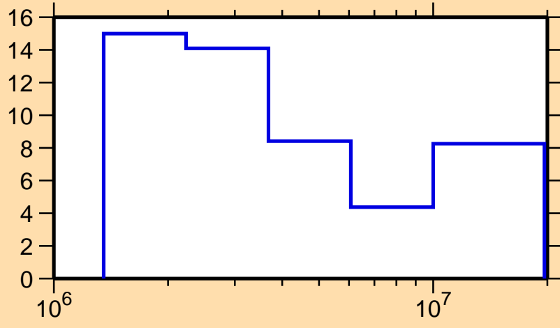
\Delta\sigma/\sigma vs. E for ^{117}\text{Te}(n,tot.)
