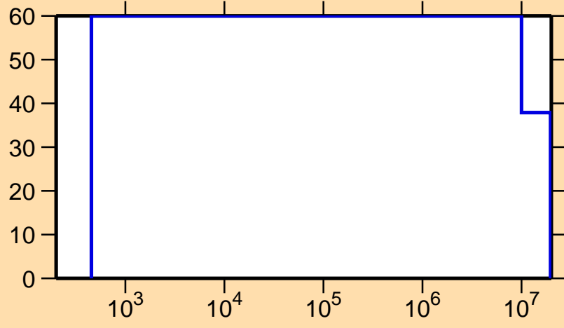
\Delta\sigma/\sigma vs. E for ^{117}\text{Te}(n,p)
