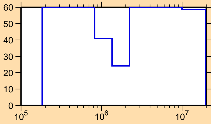
\Delta\sigma/\sigma vs. E for ^{117}\text{Te}(n,n_1)
