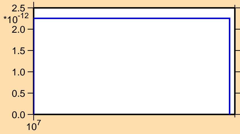
\sigma vs. E for ^{117}\text{Te}(n,nt)
