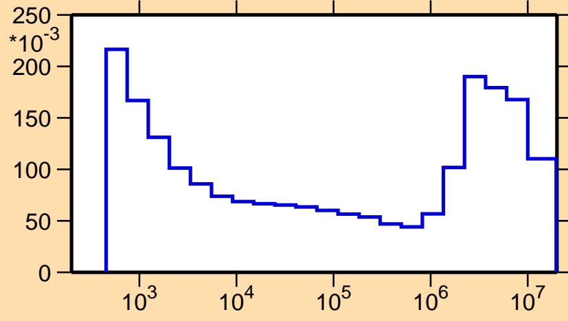
\sigma vs. E for ^{117}\text{Te}(n,p)
