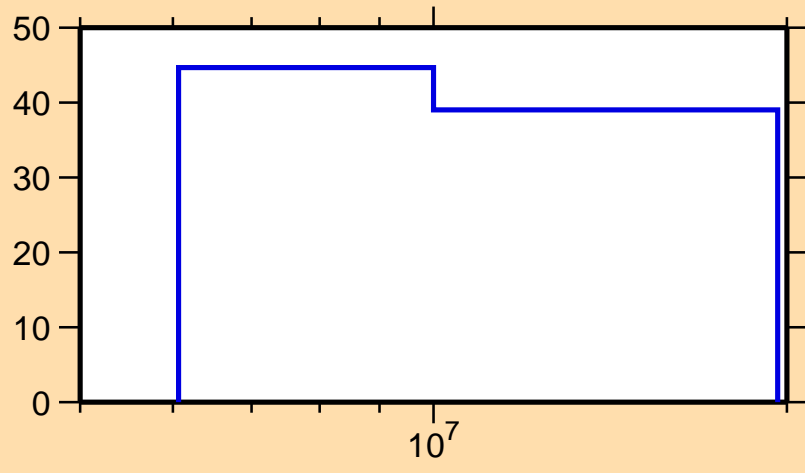
\Delta\sigma/\sigma vs. E for ^{117}\text{Te}(n,2n)
