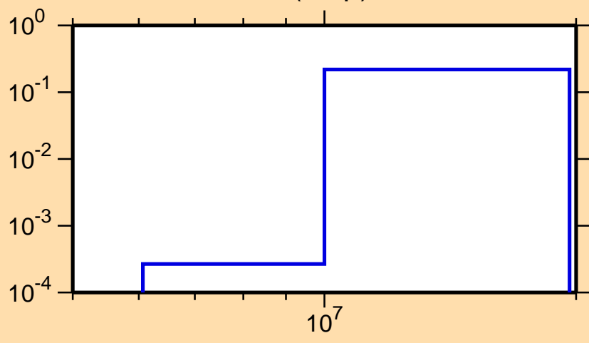
\sigma vs. E for ^{117}\text{Te}(n,np)
