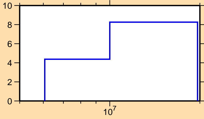
\Delta\sigma/\sigma vs. E for ^{117}\text{Te}(n,\text{tot.})
