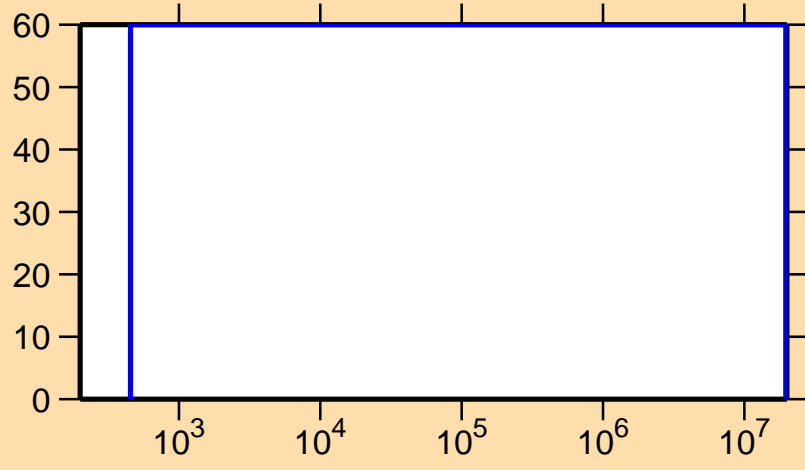
\Delta\sigma/\sigma vs. E for ^{117}\text{Te}(n,\gamma)
