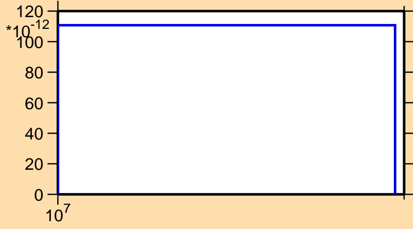
\sigma vs. E for ^{117}\text{Te} (mt 45)
