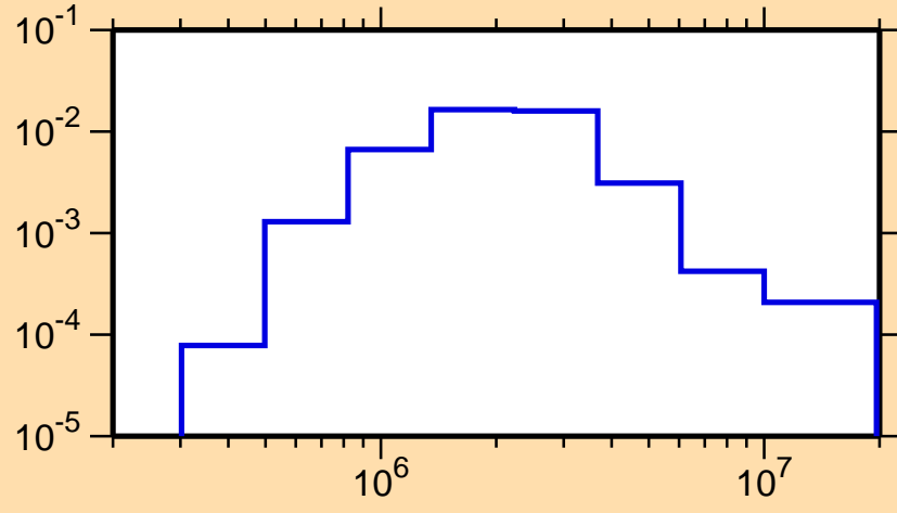
\sigma vs. E for ^{117}\text{Te}(n,n_3)
