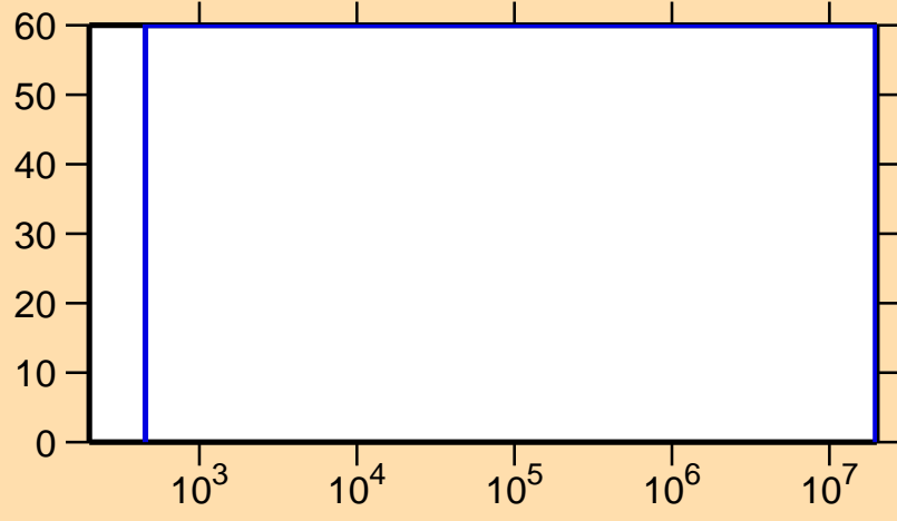
\Delta\sigma/\sigma vs. E for ^{117}\text{Te}(n,\gamma)
