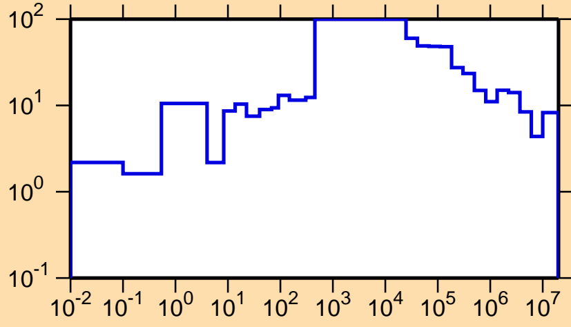
\Delta\sigma/\sigma vs. E for ^{117}\text{Te}(n,\text{tot.})
