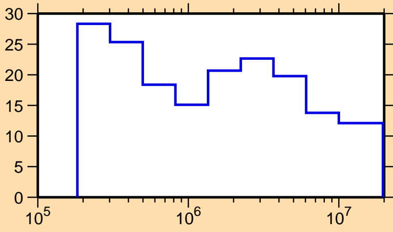
\Delta\sigma/\sigma vs. E for ^{117}\text{Te}(n,\text{el.})
