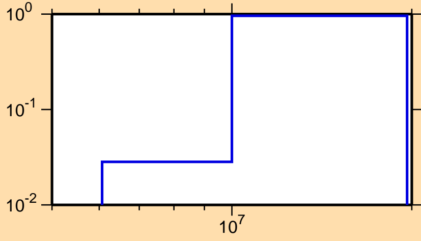
\sigma vs. E for ^{117}\text{Te}(n,2n)
