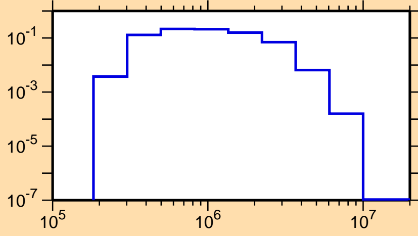
\sigma vs. E for ^{117}\text{Te}(n,n_1)
