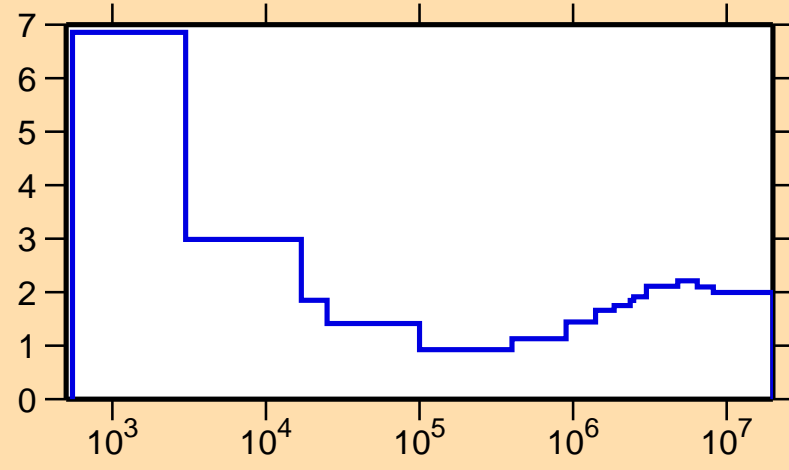
\sigma vs. E for ^{117}\text{Te}(n,\text{nonel.})
