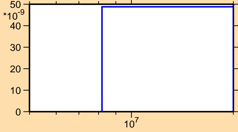
\sigma vs. E for ^{117}\text{Te}(n,pd)
