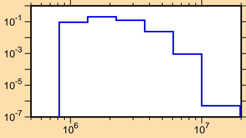
\sigma vs. E for ^{118}\text{Te}(n,n_2)
