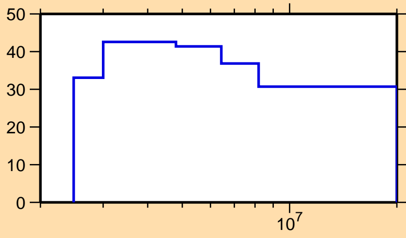
\Delta\sigma/\sigma vs. E for ^{118}\text{Te}(n, n_1)
