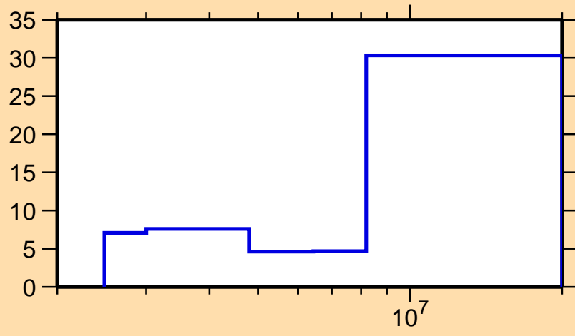
\Delta\sigma/\sigma vs. E for ^{118}\text{Te}(n,\text{inel.})
