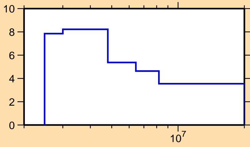
\Delta\sigma/\sigma vs. E for ^{118}\text{Te}(n,\text{nonel.})
