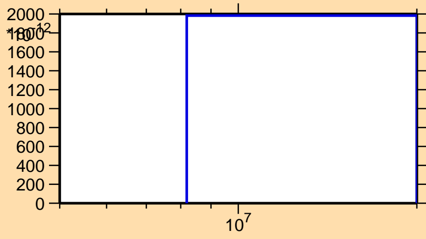
\sigma vs. E for ^{118}\text{Te}(n,\text{nd})
