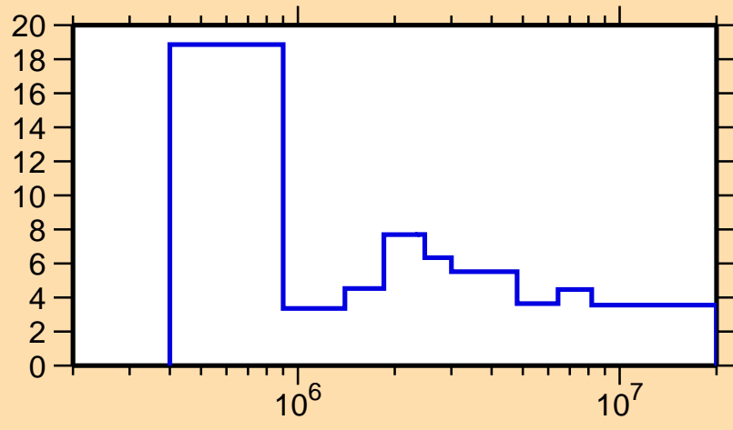
\Delta\sigma/\sigma vs. E for ^{118}\text{Te}(n,\text{tot.})
