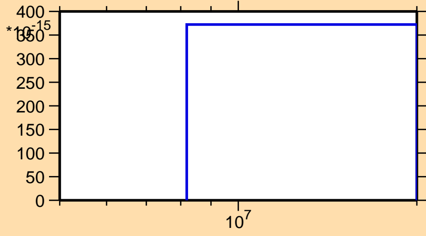
\sigma vs. E for ^{118}\text{Te}(n,\text{pt})
