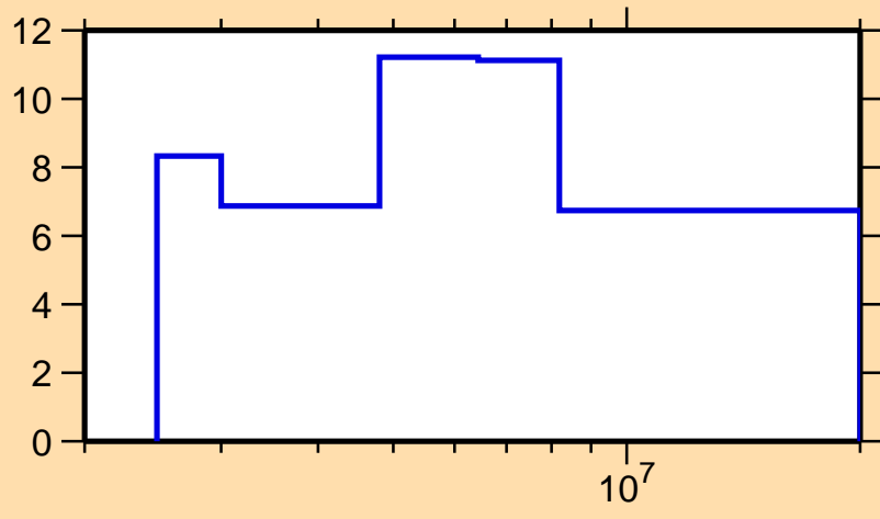
\Delta\sigma/\sigma vs. E for ^{118}\text{Te}(n,\text{el.})
