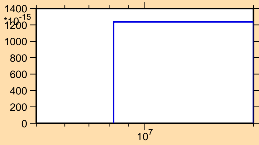
\sigma vs. E for ^{118}\text{Te}(\text{mt117})
