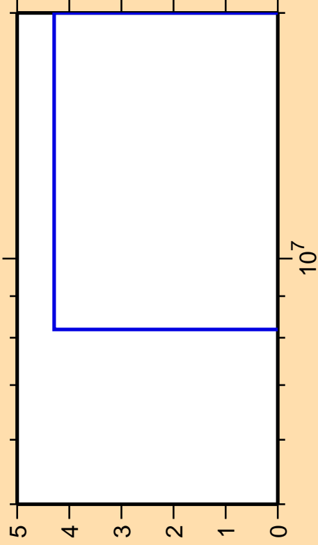
\Delta\sigma/\sigma vs. E for ^{118}\text{Te}(\text{mt117})
