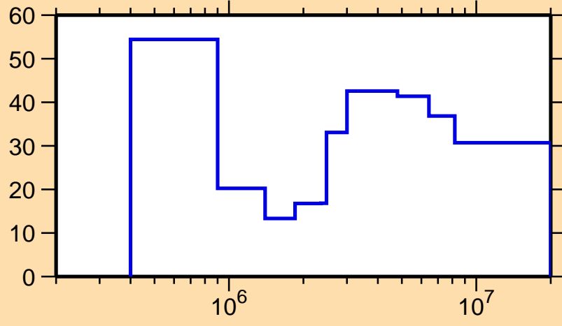
\Delta\sigma/\sigma vs. E for ^{118}\text{Te}(n,n_1)
