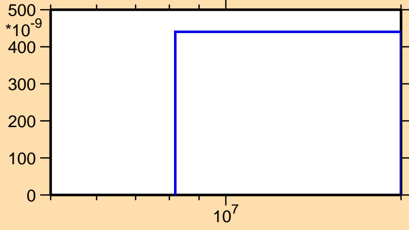
\sigma vs. E for ^{118}\text{Te}(n,3n)
