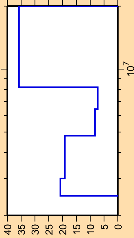
\Delta\sigma/\sigma vs. E for ^{118}\text{Te}(n,n\text{cont.})
