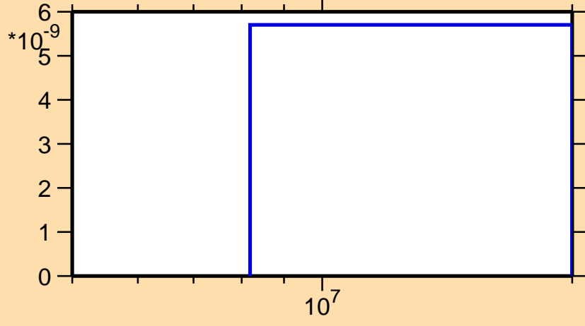
\sigma vs. E for ^{118}\text{Te}(n,pd)
