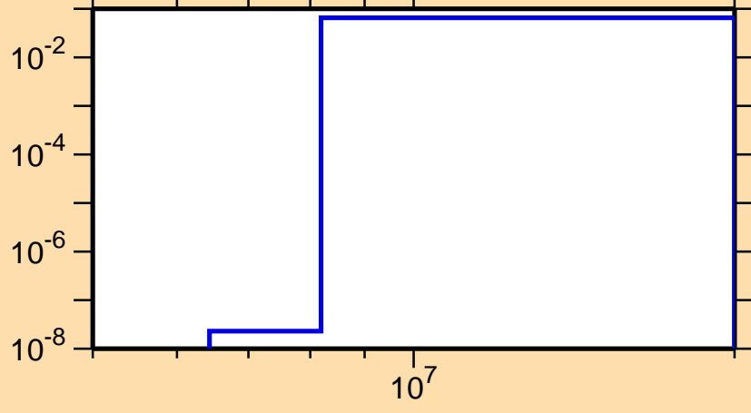
\sigma vs. E for ^{118}\text{Te}(n,np)
