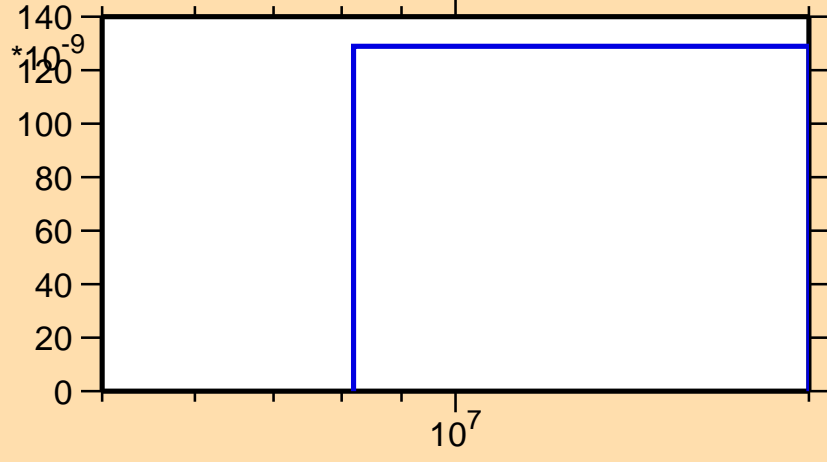
\sigma vs. E for ^{118}\text{Te}(n,p\alpha)
