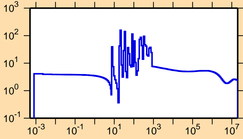
\sigma vs. E for ^{119}\text{Te}(n,\text{el.})
