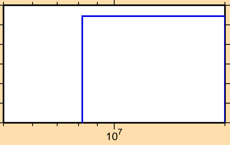
\sigma vs. E for ^{119}\text{Te}(n,nt)
