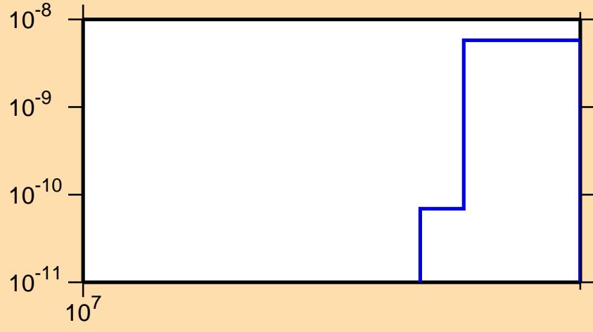
\sigma vs. E for ^{119}\text{Te}(n,\text{pt})
