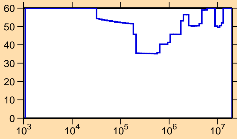
\Delta\sigma/\sigma vs. E for ^{119}\text{Te}(n,\gamma)
