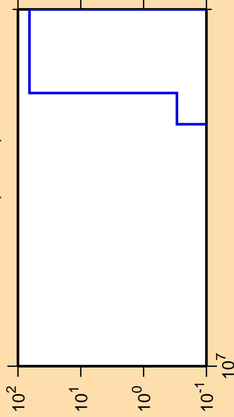
\Delta\sigma/\sigma vs. E for ^{119}\text{Te} (mt 45)
