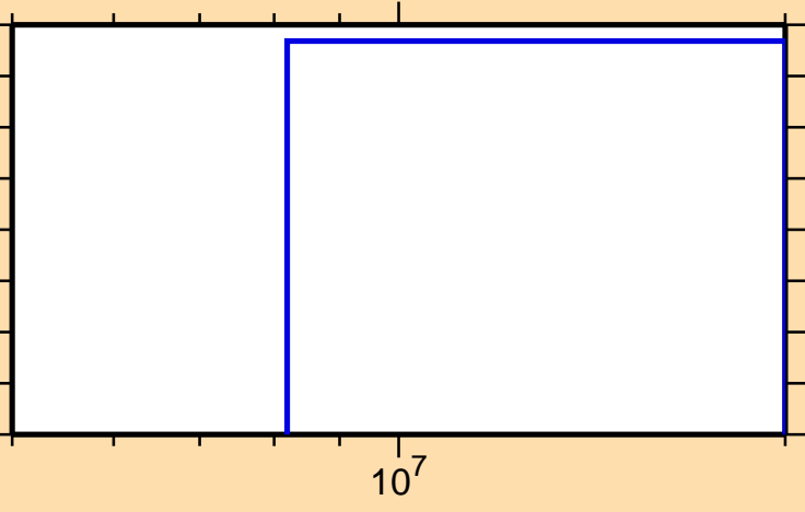
\sigma vs. E for ^{119}\text{Te}(\text{mt117})
