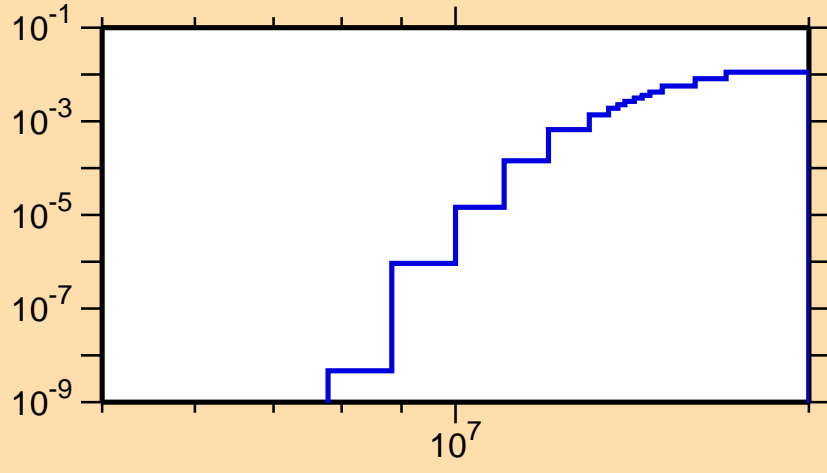
\sigma vs. E for ^{120}\text{Te}(n,d)
