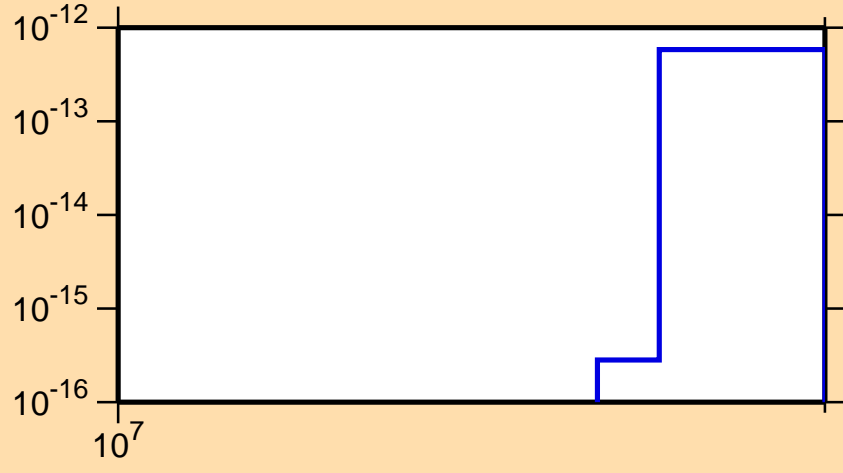
\sigma vs. E for ^{120}\text{Te} (mt 45)
