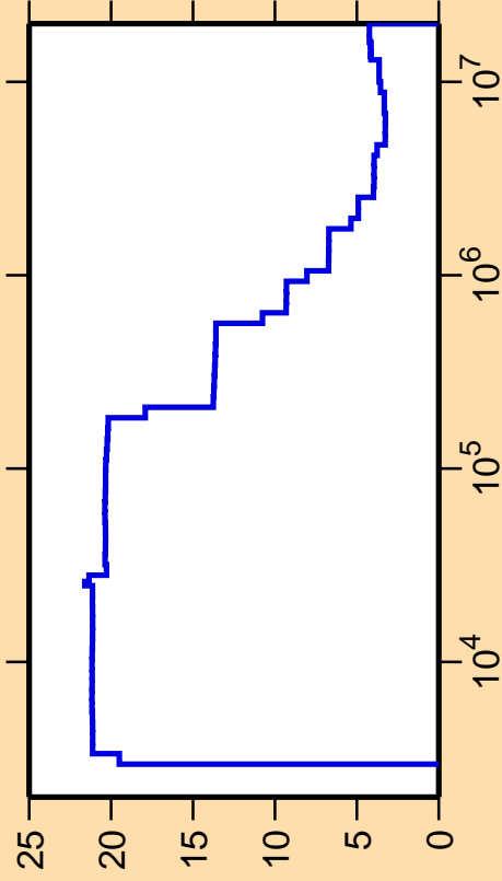
\Delta\sigma/\sigma vs. E for ^{120}\text{Te}(n,\text{nonel.})
